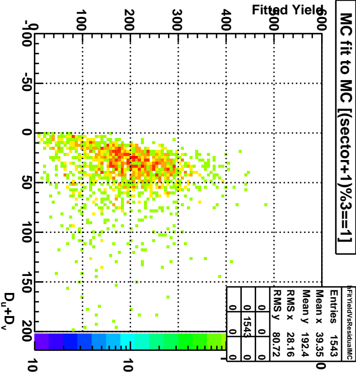
MC fit to Data [(sector+1)%3==1]
