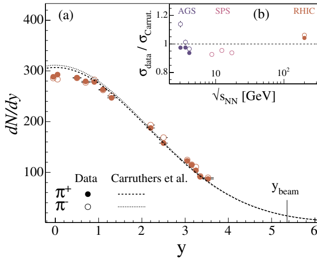
FIG. 4 (color online). Comparison dN/dy(\pi) and Landau's prediction at \sqrt{s_{NN}} = 200 GeV (a), and ratio \sigma_{N(\pi)}/\sigma_{\text{Carruth.}} as a function of \sqrt{s_{NN}} (b). Errors are statistical.
