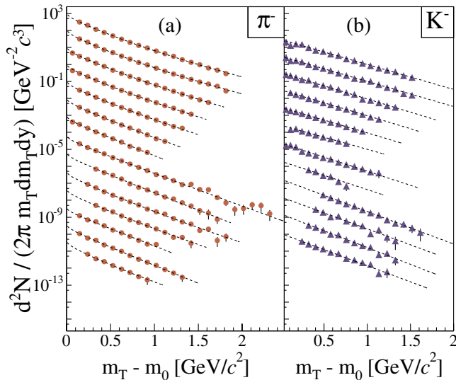
FIG. 1 (color online). Invariant transverse mass m_T - m_0 spectra of \pi^- (a) and K^- (b) from y \sim 0 (top) to y \sim 3.5 (bottom). Dashed lines are fits to the data, namely, a power law in p_T for pions and an exponential in m_T - m_0 for kaons. Errors are statistical. Spectra have been rescaled by powers of 10 for clarity.
