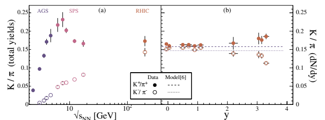
FIG. 3 (color online). Full phase-space K/\pi ratios as a function of \sqrt{s_{NN}} (a) and rapidity systematics at \sqrt{s_{NN}} = 200 GeV (b). The dashed and dotted lines in (b) are predictions of the statistical model [6]. Errors are statistical and systematic in (a), and only statistical in (b). AGS data are from [18,19]; SPS data are from [13,20,21]. Data points at \sqrt{s_{NN}} = 6.3 and 7.6 GeV [20,21] are preliminary.
