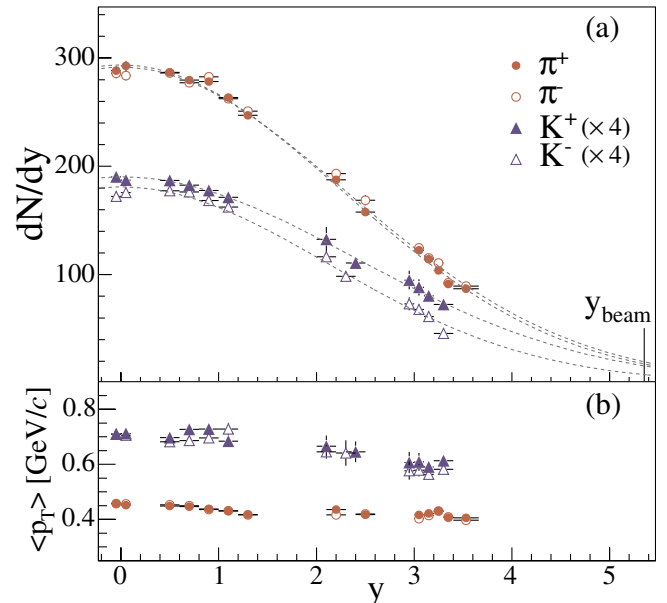
FIG. 2 (color online). Pion and kaon rapidity densities (a) and their mean transverse momentum \langle p_T \rangle (b) as a function of rapidity. Errors are statistical. The kaon yields were multiplied by 4 for clarity. The dashed lines in (a) are Gaussian fits to the dN/dy distributions (see text).
