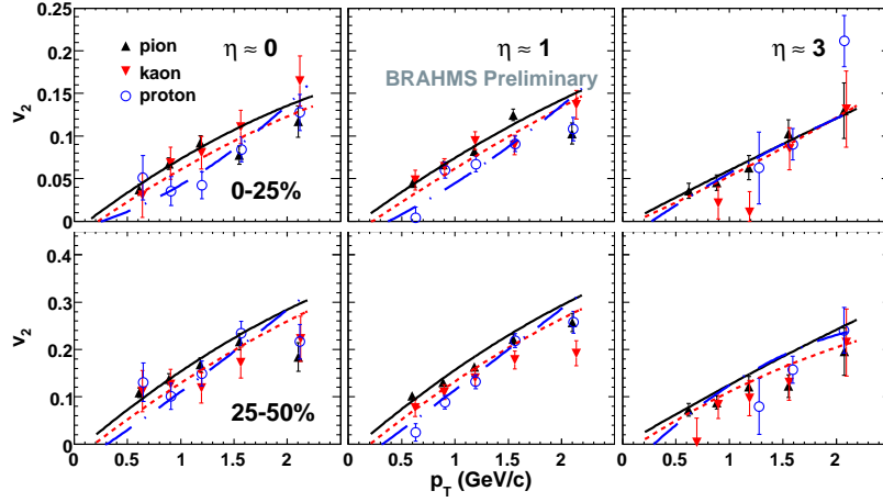
Figure 2: Identified particle v_2(p_T) for central and mid-central events for \eta \approx 0, 1 and 3 . The curves show 3D Hydro+Cascade calculations [3] for pions(solid), kaons(short dash), and protons (long dash).
