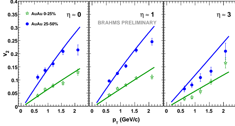
Figure 1: Charge-hadron v_2(p_T) for central and mid-central events for \eta \approx 0, 1 and 3 . The curves show 3D Hydro+Cascade calculations [3].
