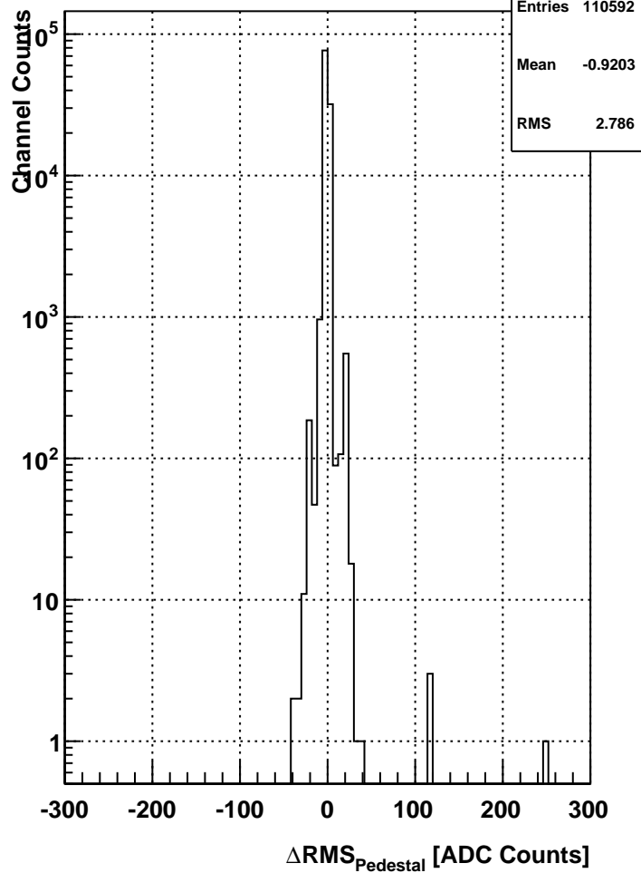
hist_rmsPedDiff_TimeBin2_1D
