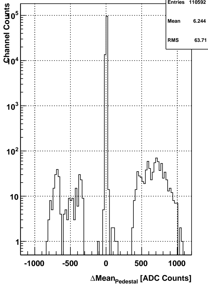
hist_meanPedDiff_TimeBin2_1D
