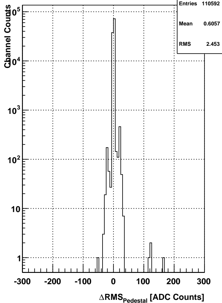
hist_rmsPedDiff_TimeBin4_1D
