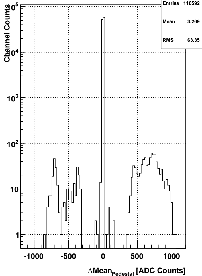
hist_meanPedDiff_TimeBin4_1D
