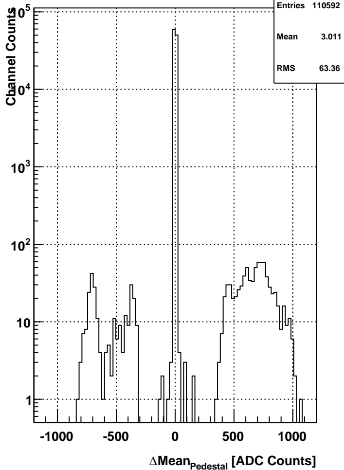
hist_meanPedDiff_TimeBin7_1D
