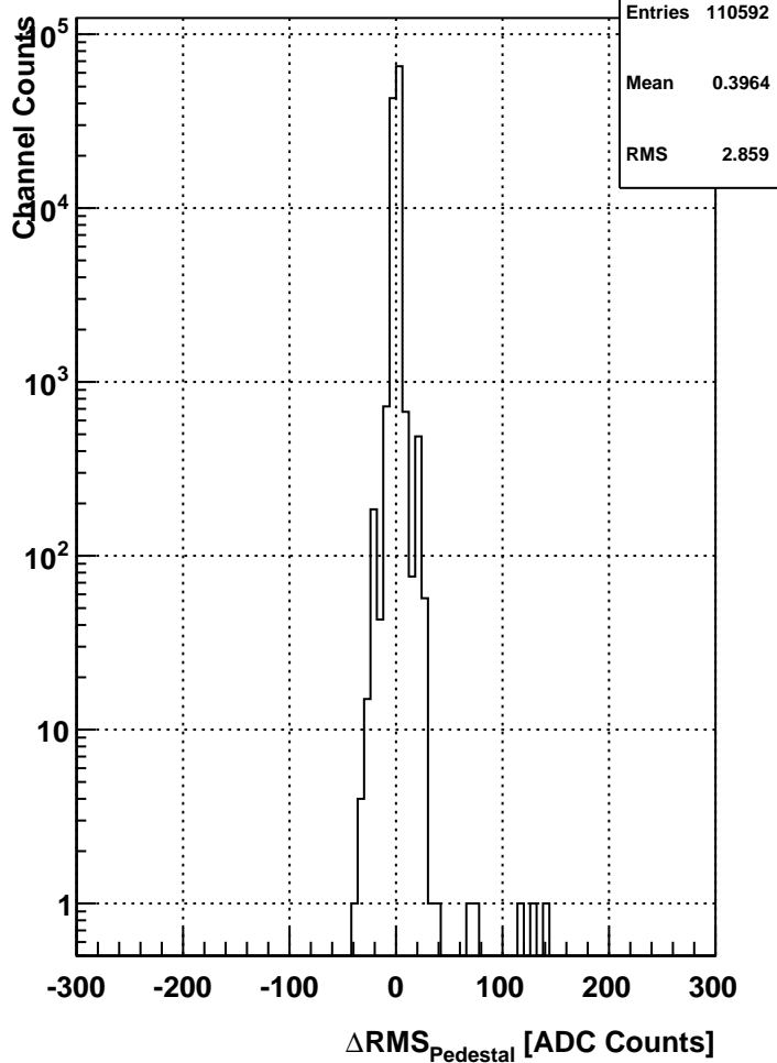
hist_rmsPedDiff_TimeBin7_1D
