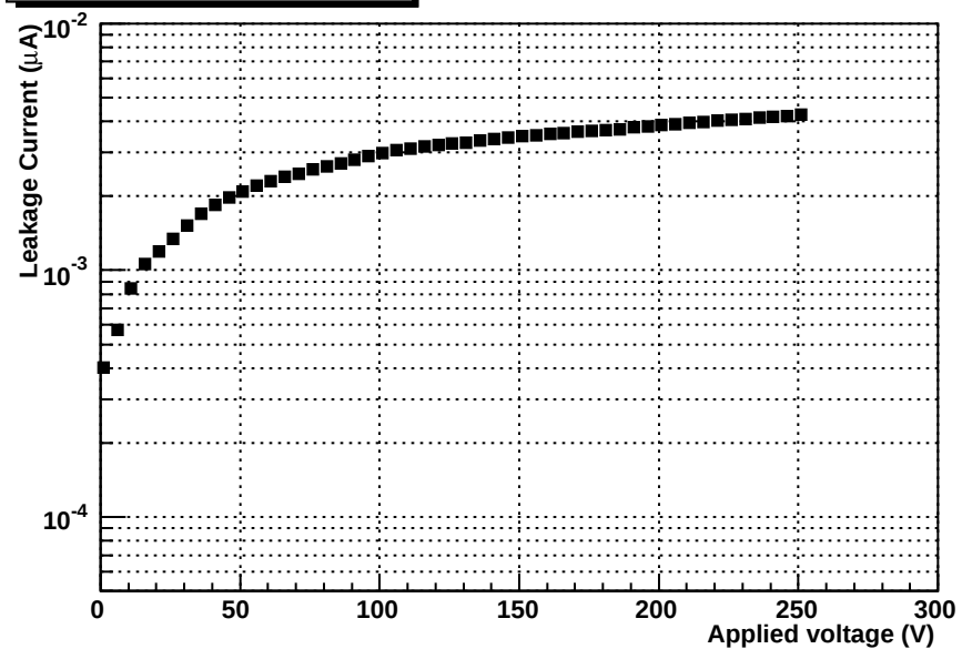
pC-CNI Si #1433-D1-GR
