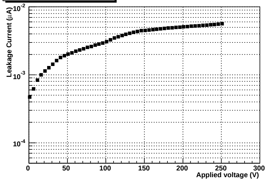
pC-CNI Si #1433-D8-GR
