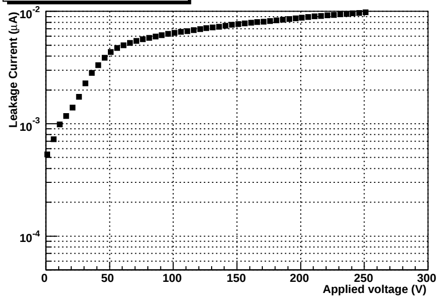
pC-CNI Si #1433-D7-GR
