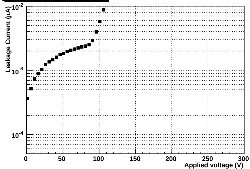
pC-CNI Si #1433-D2-GR
