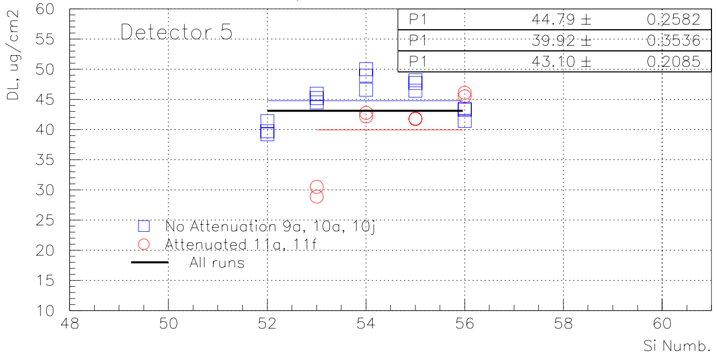
Dead Layer for Individual Detectors
