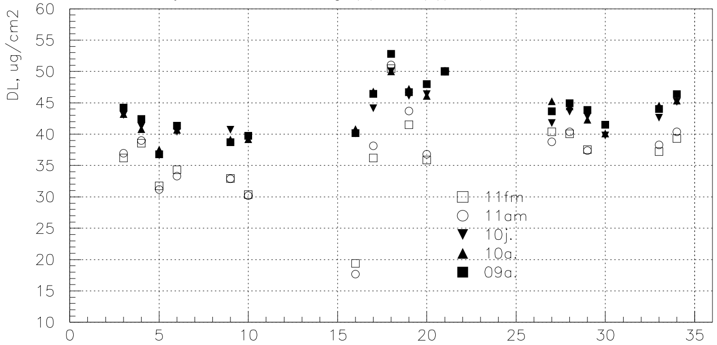
Dead Layer Thickness to Bring t(1/\sqrt{e}) Slope to Calibr. Coefs.
