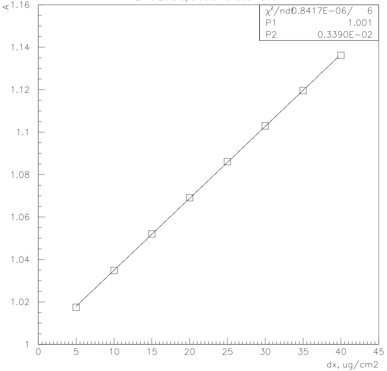
Ei vs Ed Slope as a Function of dx
