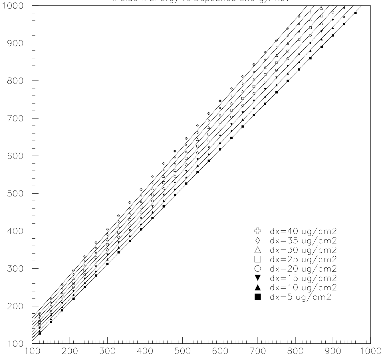
Incident Energy vs Deposited Energy, KeV
