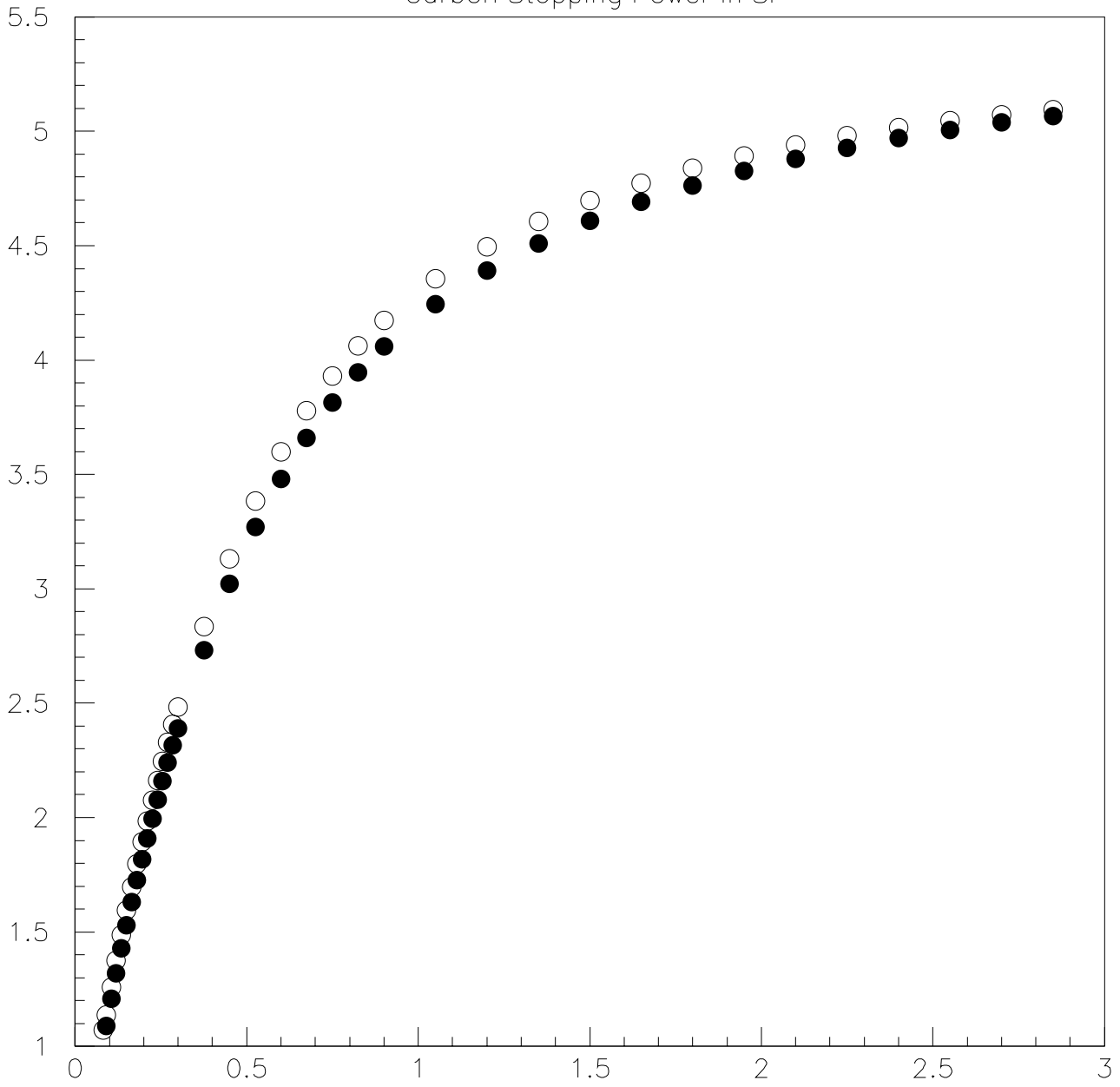
Carbon Stopping Power in Si
