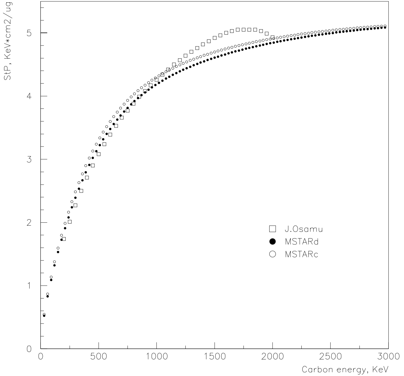
Carbon Stopping Power in Si
