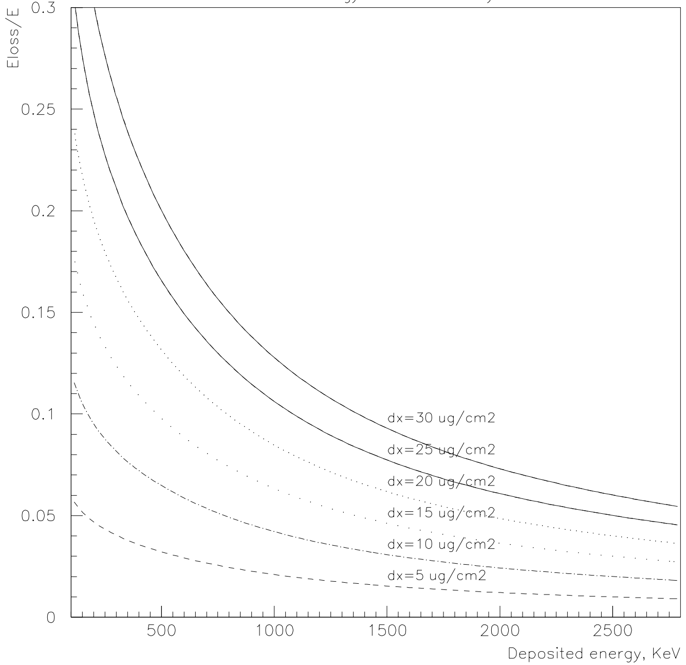
Relative Energy Loss in Dead Layer
