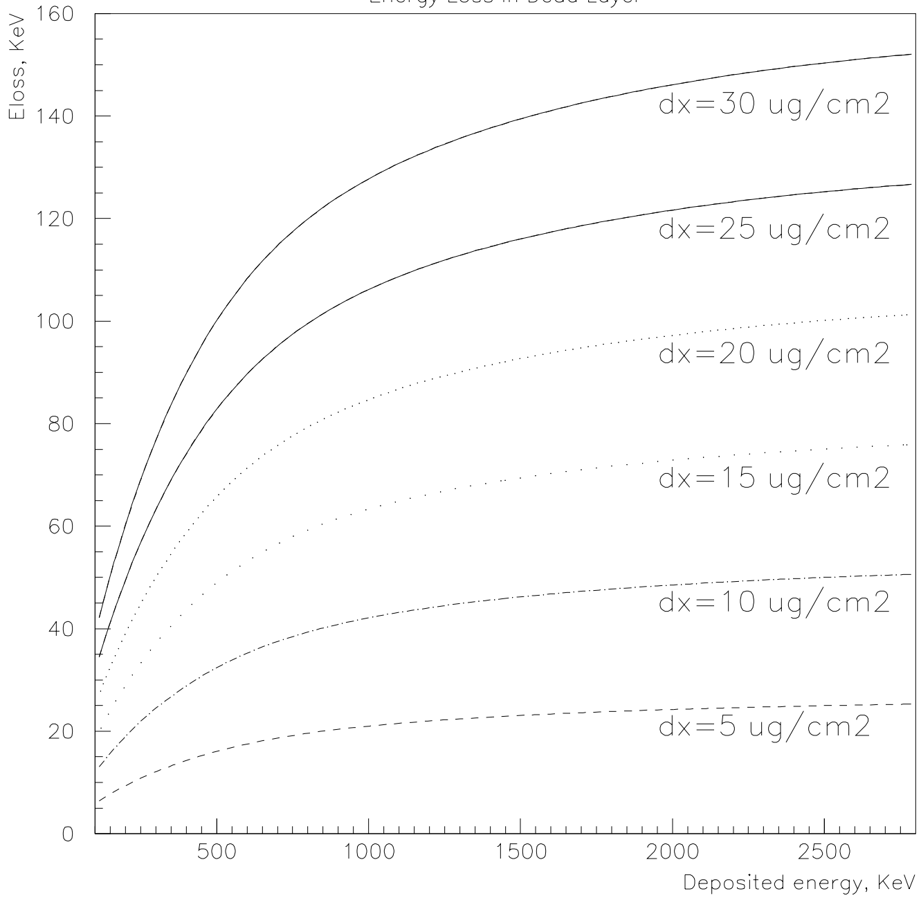
Energy Loss in Dead Layer
