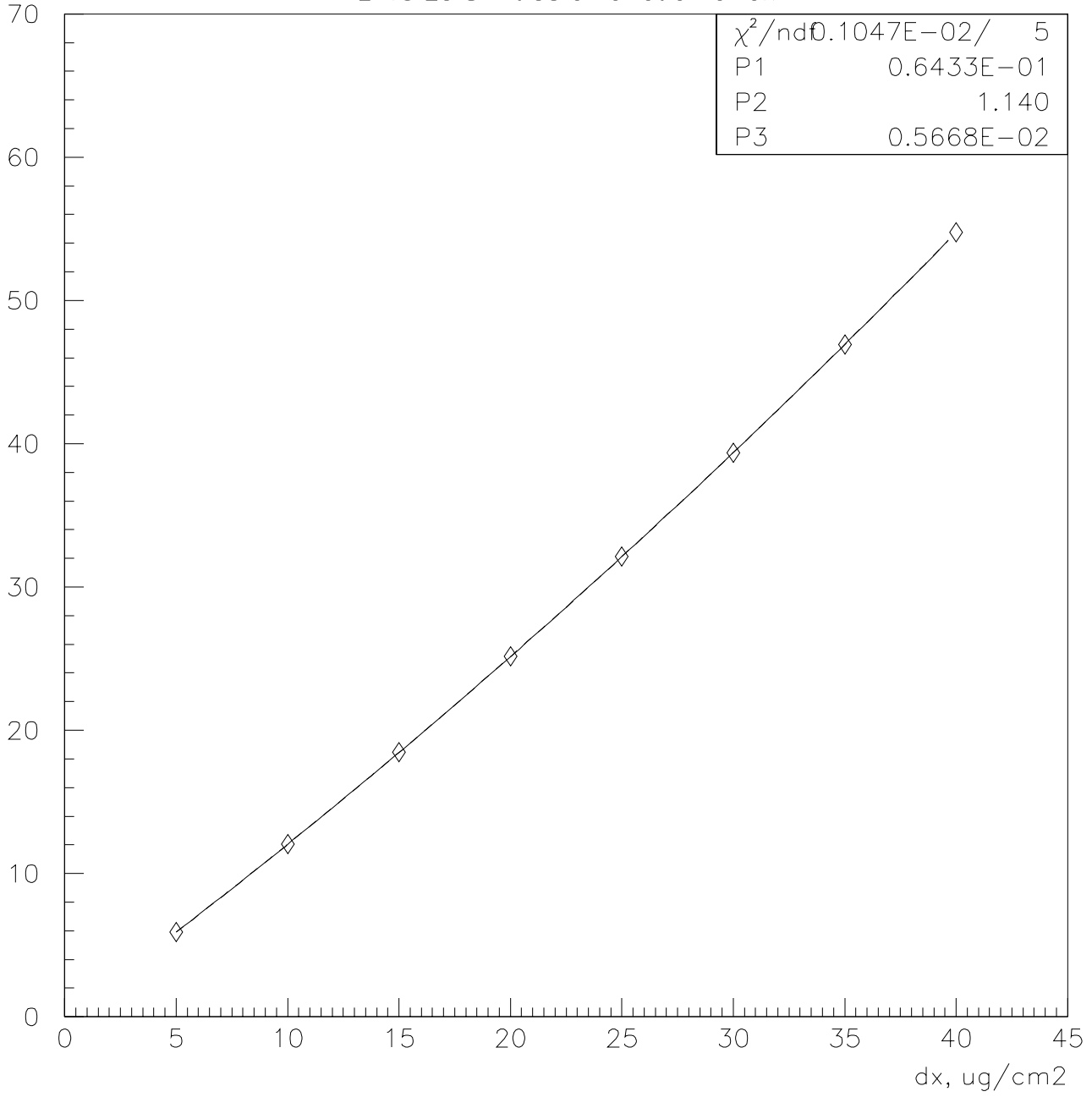
Ei vs Ed Shift as a Function of dx
