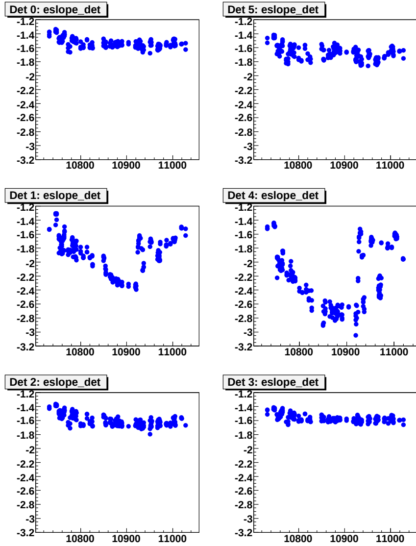
Figure 64. The same as Fig. 63, but for \sqrt{s}=200 GeV measurements.
