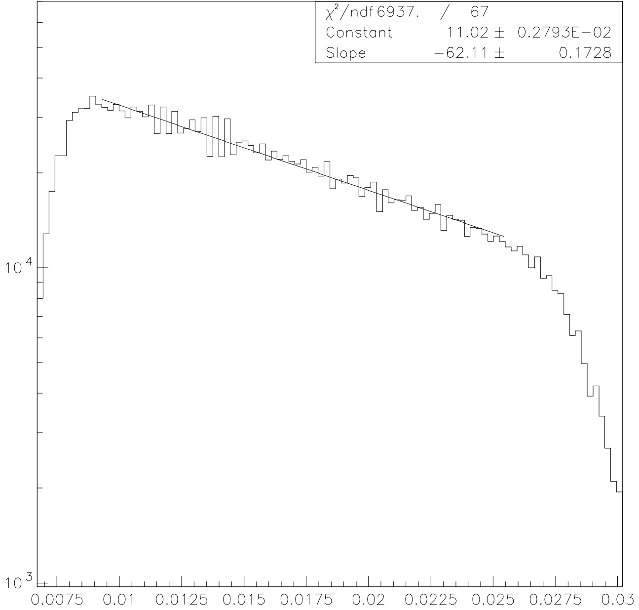
-t Spectrum from IEE for Run 10009a
