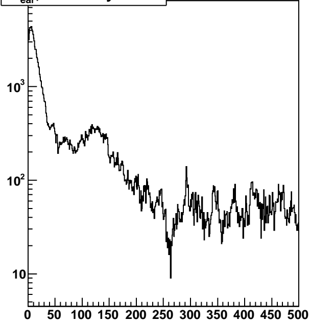
t-t_{\text{ear}} , nHits/tray/ev>25
