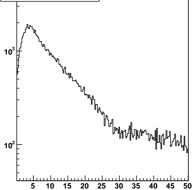
t-t_{\text{ear}}, n\text{Hits}/\text{tray}/\text{ev}>25
