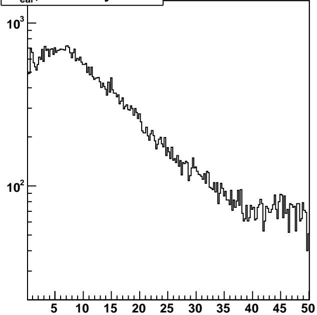
t-t_{\text{ear}}, n\text{Hits}/\text{tray}/\text{ev}>25
