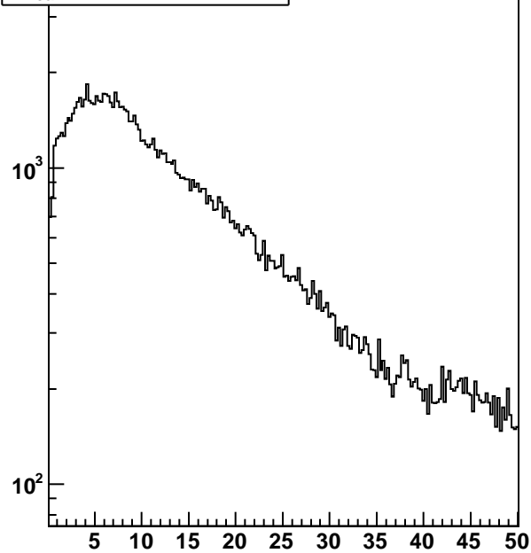
t-t_{\text{ear}} , nHits/tray/ev>25
