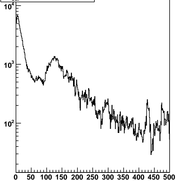
t-t_{\text{ear}} , nHits/tray/ev>25
