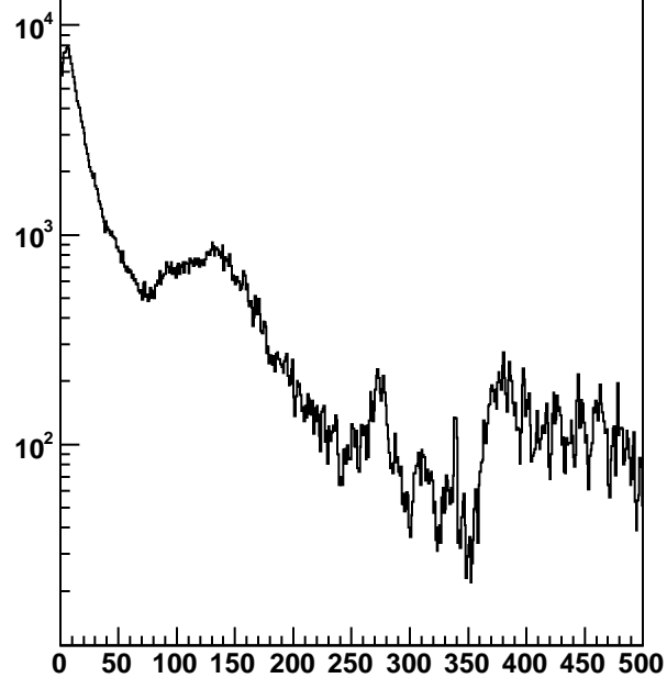
t-t_{\text{ear}}, n\text{Hits}/\text{tray}/\text{ev}>25
