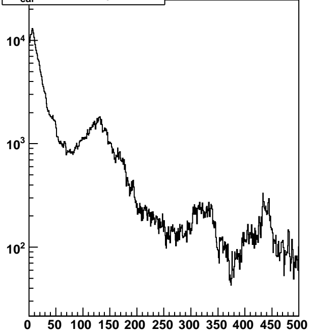
t-t_{\text{ear}} , nHits/tray/ev>25
