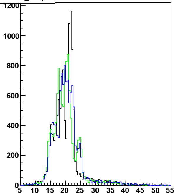
hmtdhitz_totm_strip1_norm
