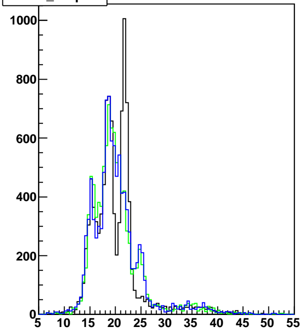
hmtdhitz_totm_strip12_norm
