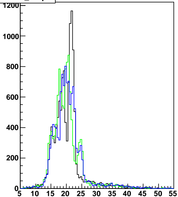
hmtdhitz_totm_strip1
