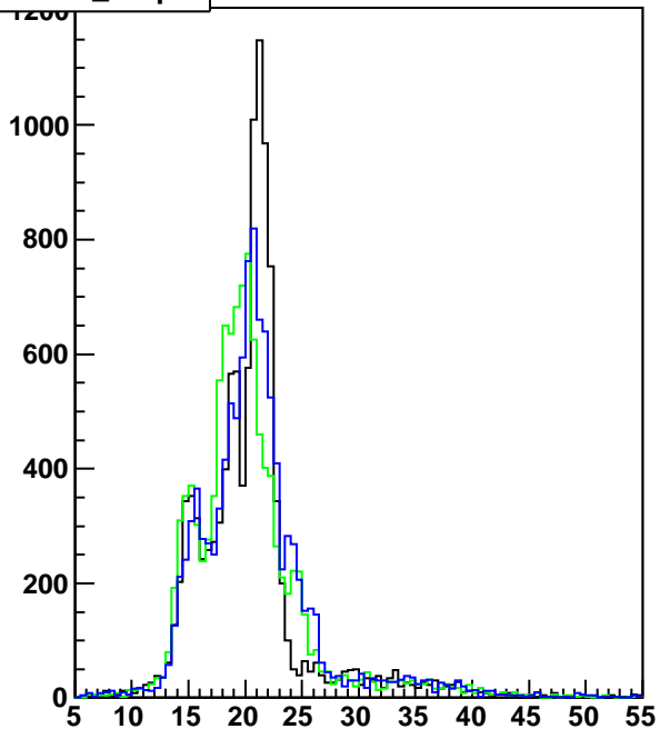
hmtdhitz_totm_strip6
