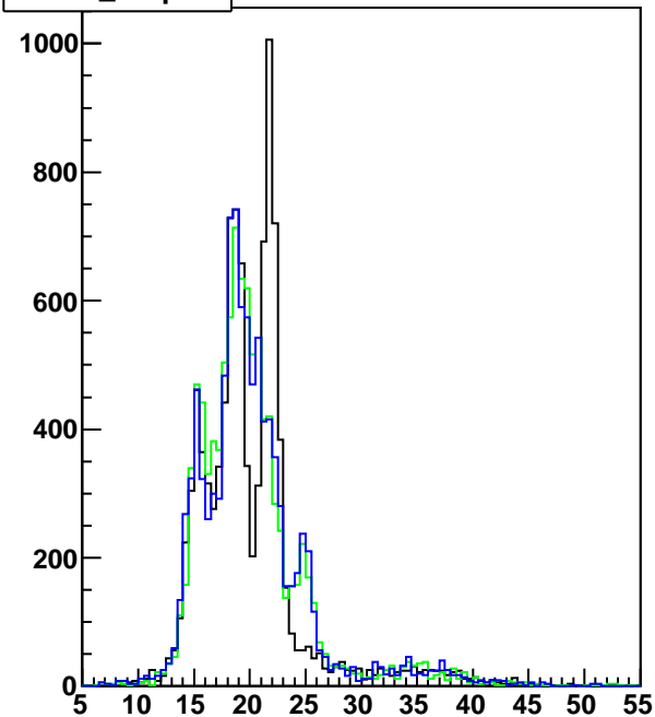
hmtdhitz_totm_strip12
