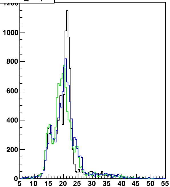
hmtdhitz_totm_strip6_norm
