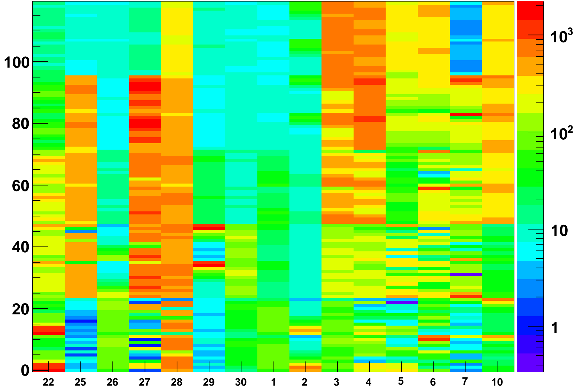
Rate (Hz) vs (BL,strip-posn), Run=14160
