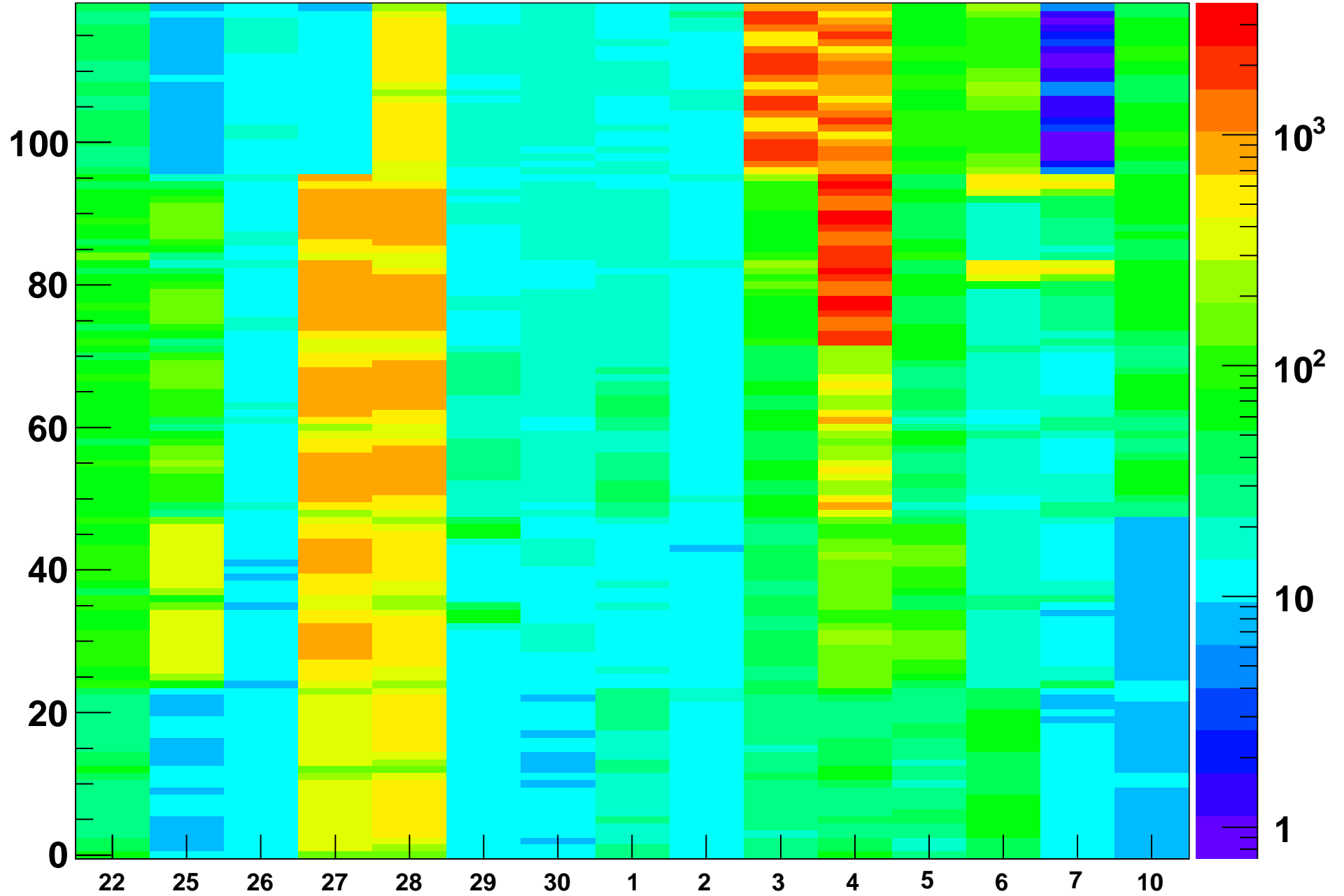
Rate (Hz) vs (BL,strip-posn), Run=14083
