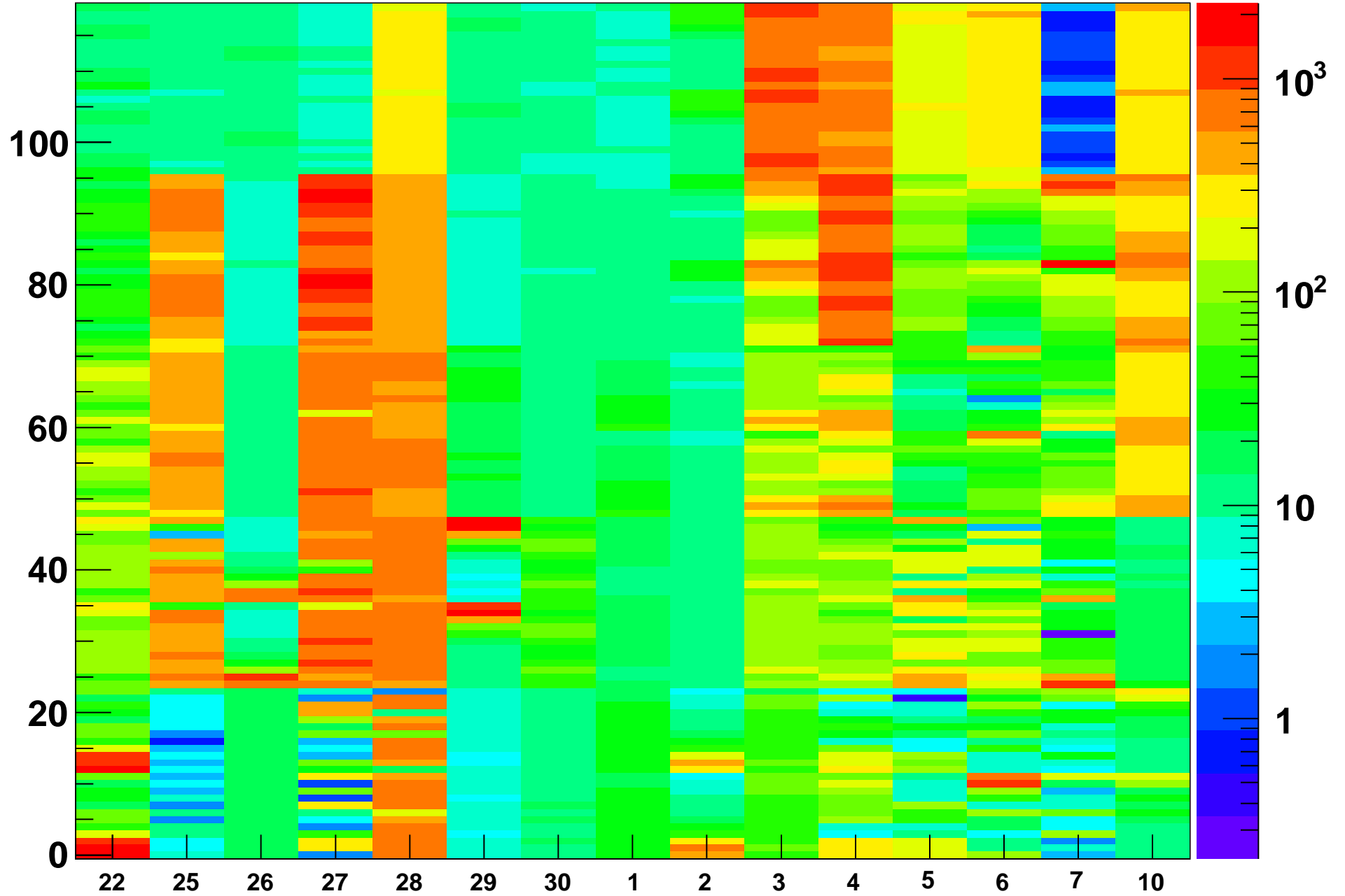
Rate (Hz) vs (BL,strip-posn), Run=14143
