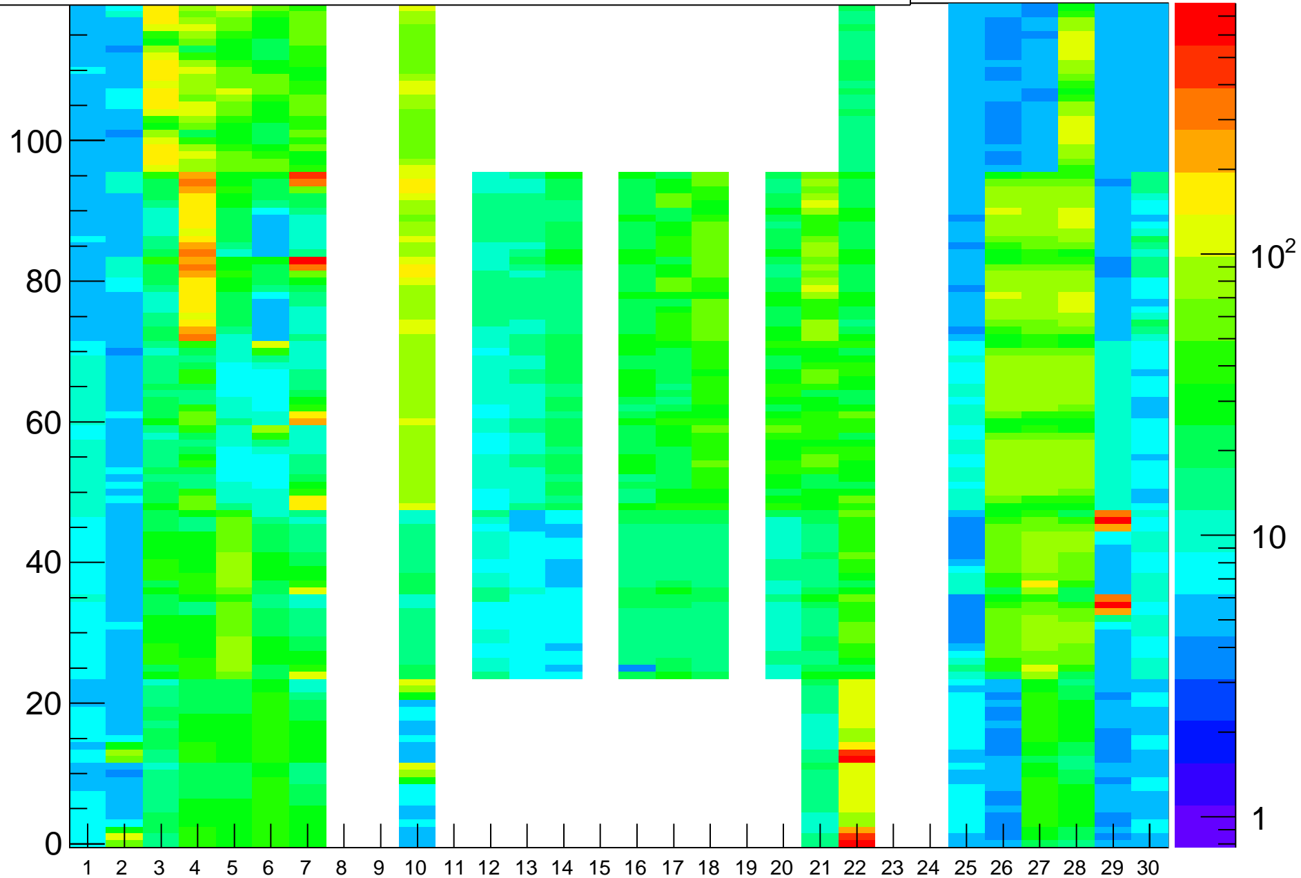
Rate (Hz) vs (BL,strip-posn), Run=15024
