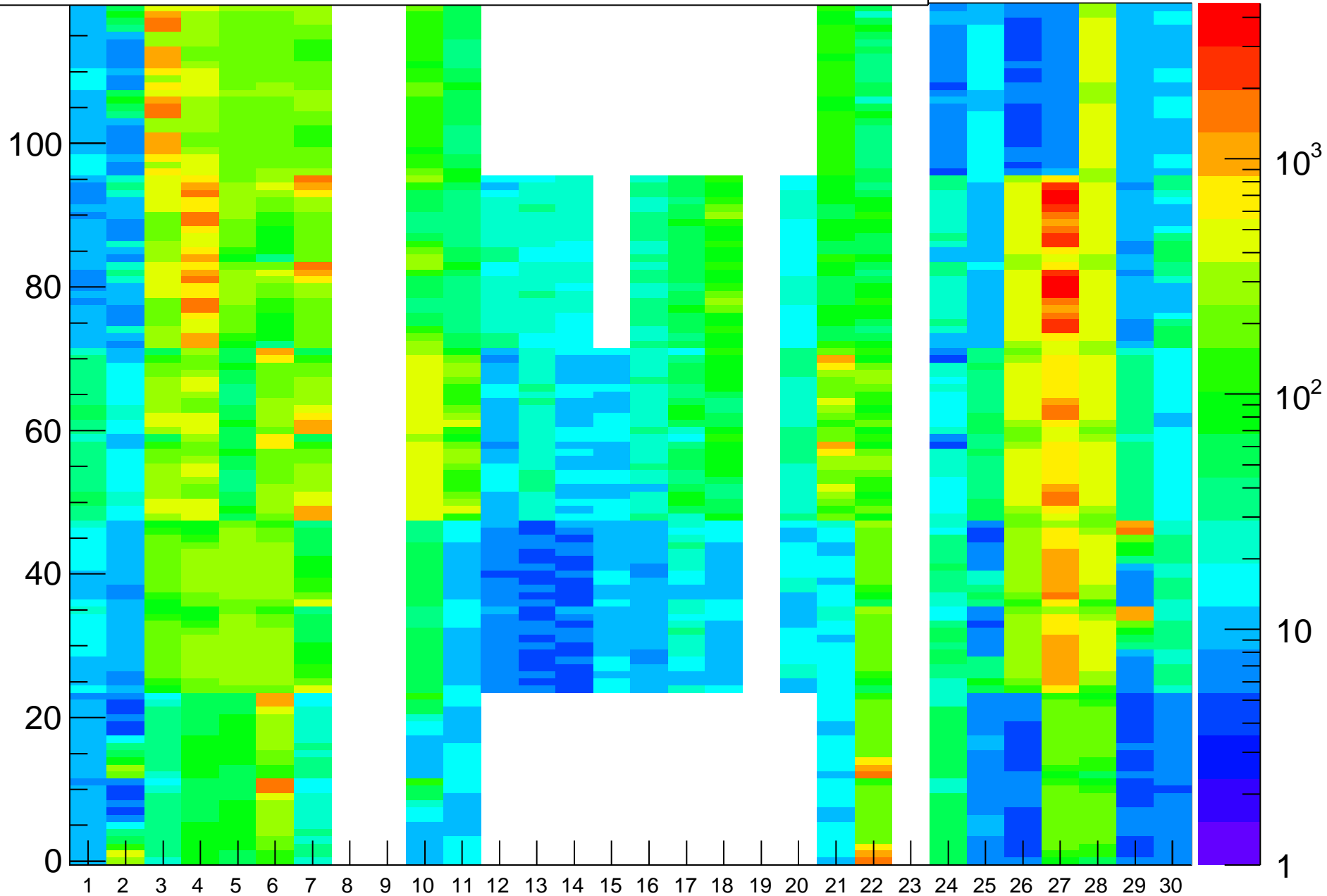
Rate (Hz) vs (BL,strip-posn), Run=15057
