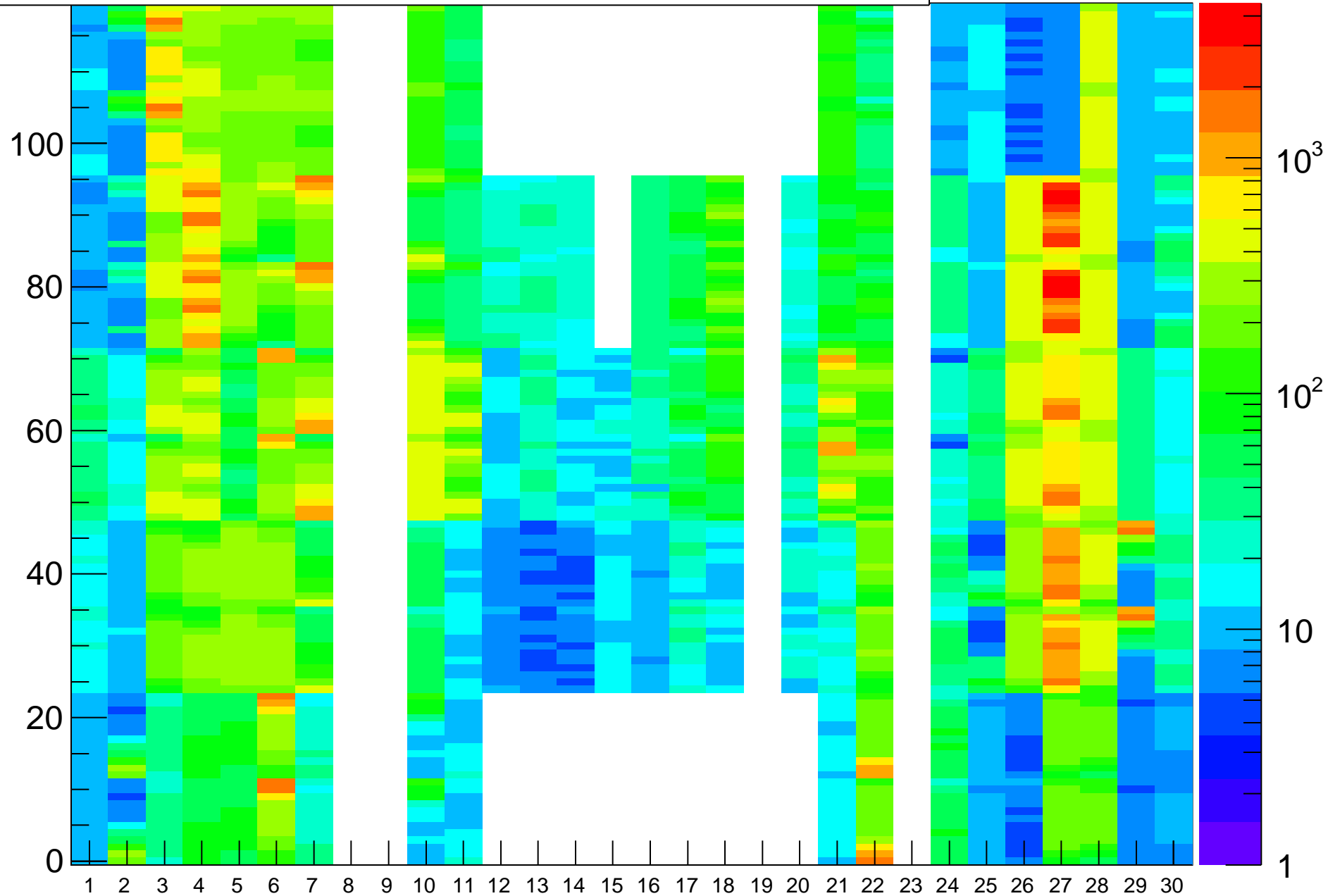
Rate (Hz) vs (BL,strip-posn), Run=15058
