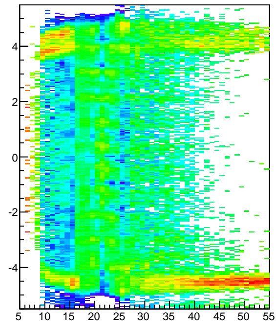
hmtdhitz_totm_strip12_norm
