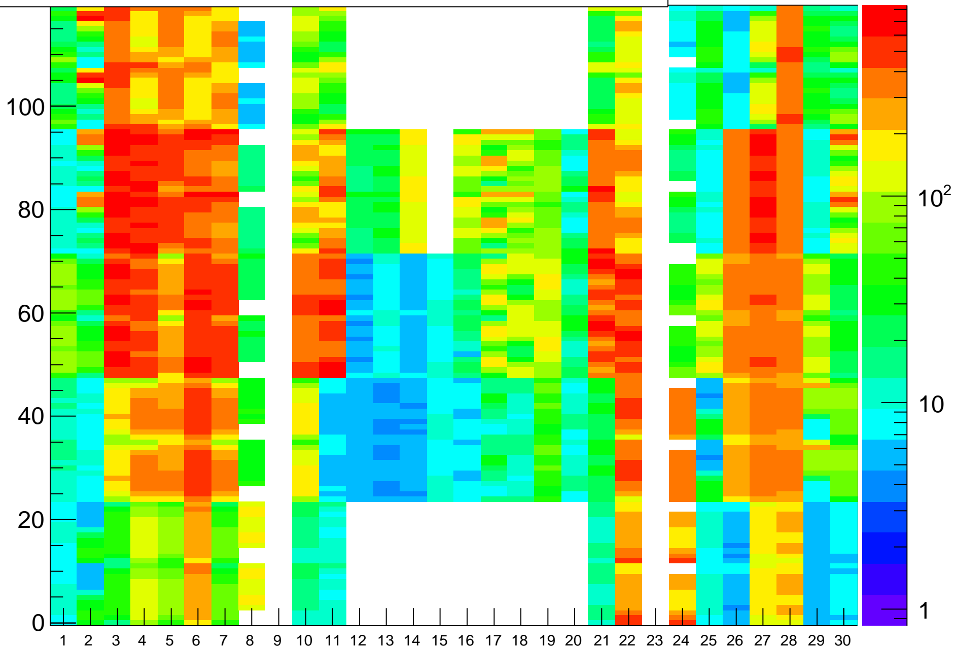
Rate (Hz) vs (BL,strip-posn), Run=15120080
