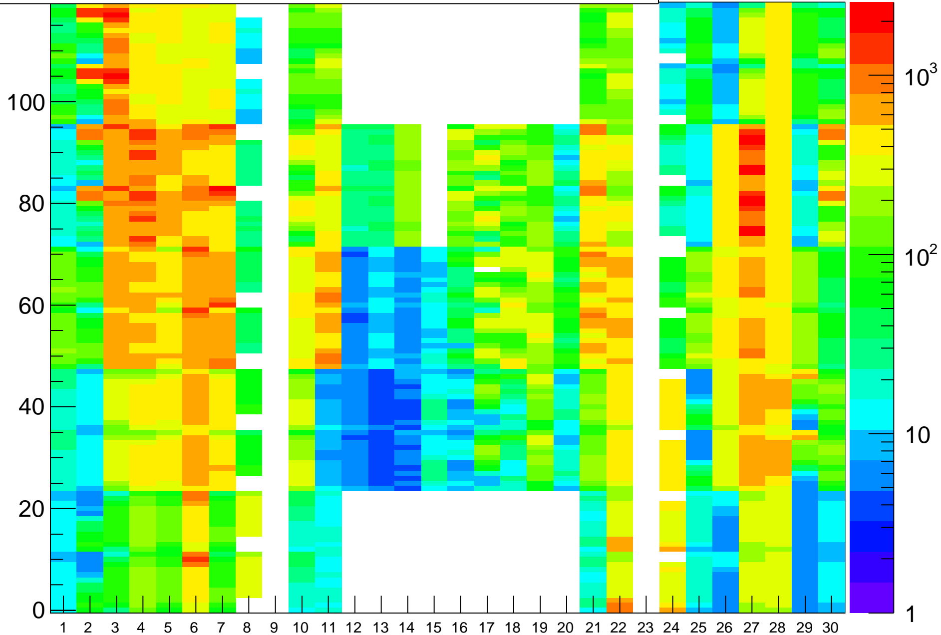
Rate (Hz) vs (BL,strip-posn), Run=15128
