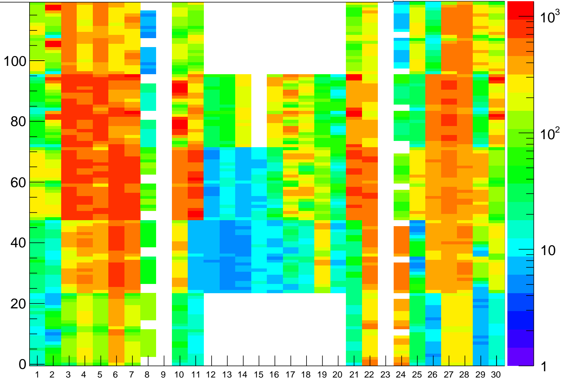
Rate (Hz) vs (BL,strip-posn), Run=15145
