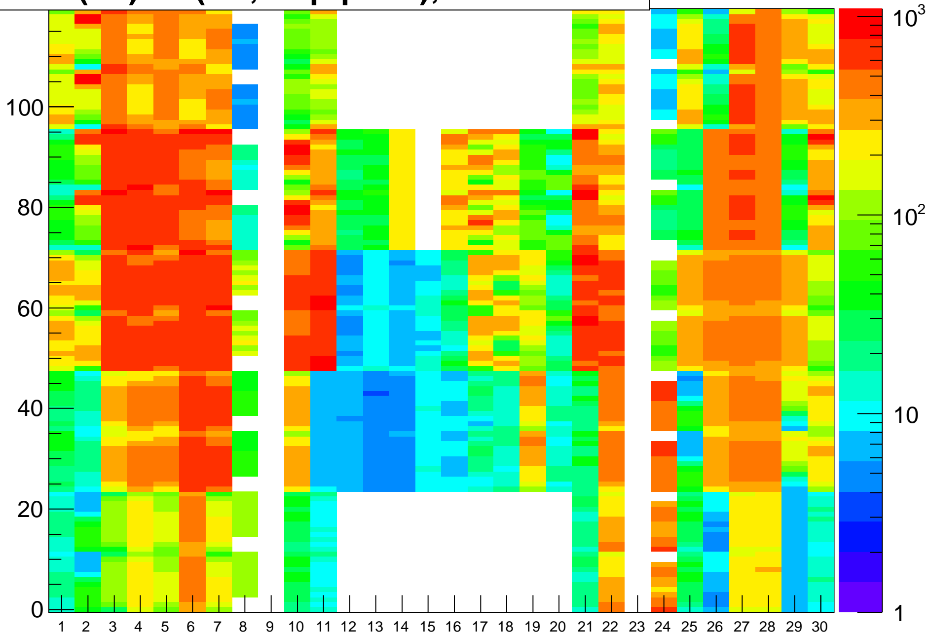
Rate (Hz) vs (BL,strip-posn), Run=15149
