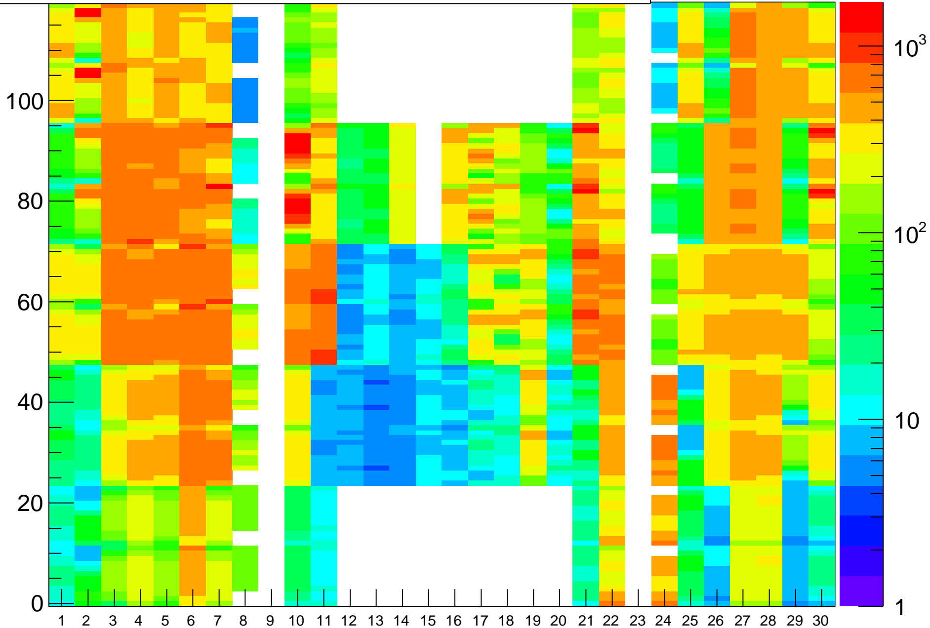
Rate (Hz) vs (BL,strip-posn), Run=15158
