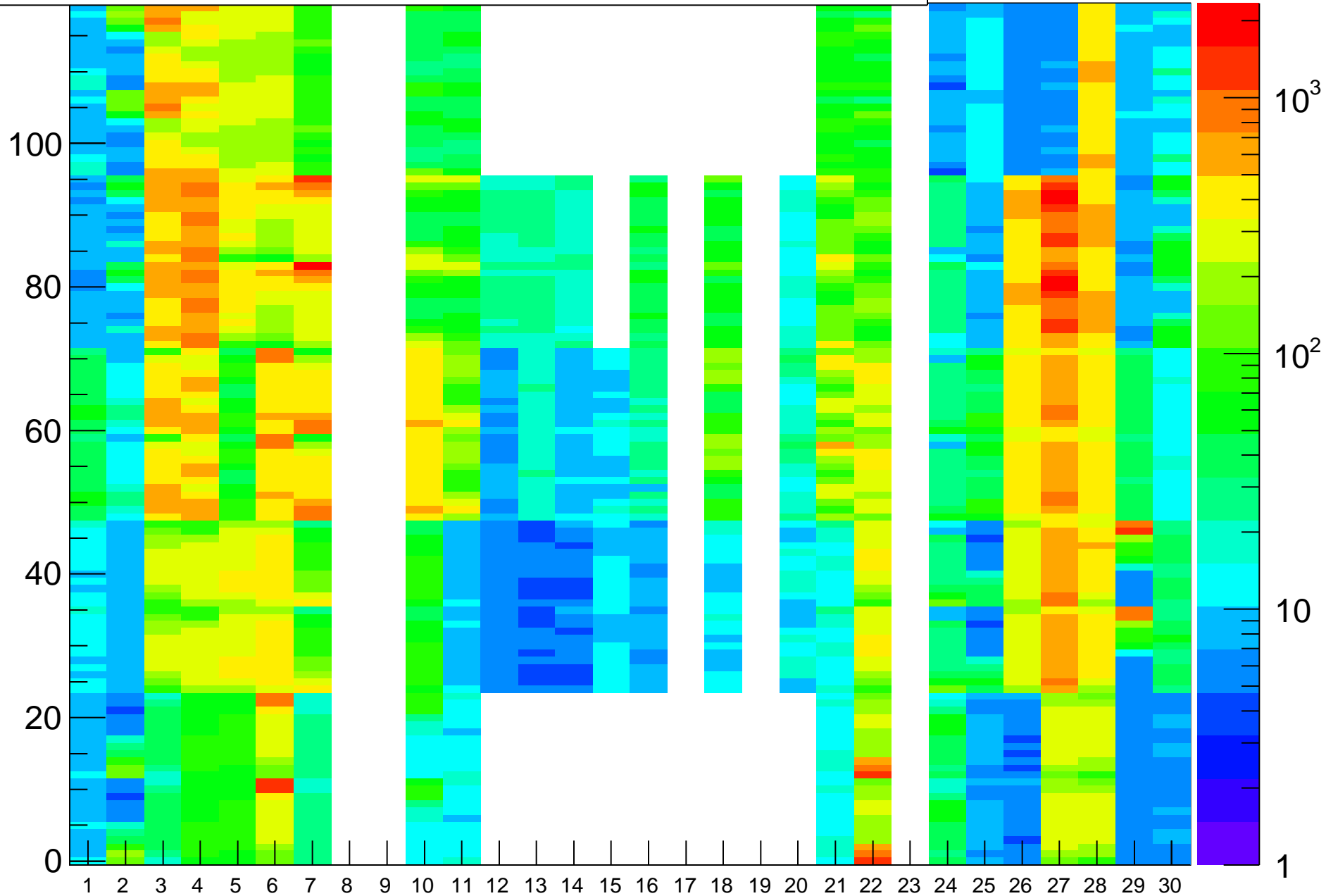
Rate (Hz) vs (BL,strip-posn), Run=15077
