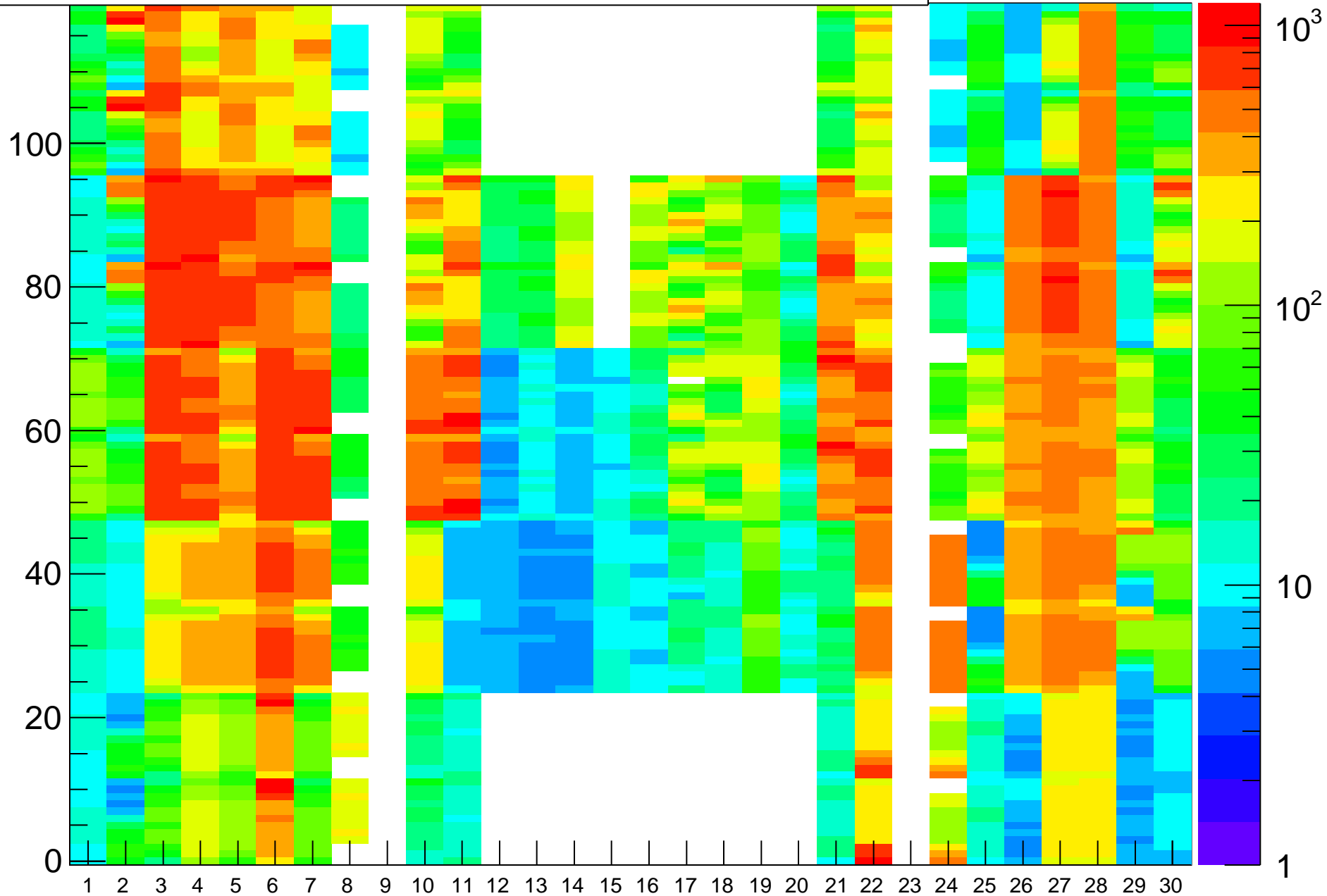
Rate (Hz) vs (BL,strip-posn), Run=15122
