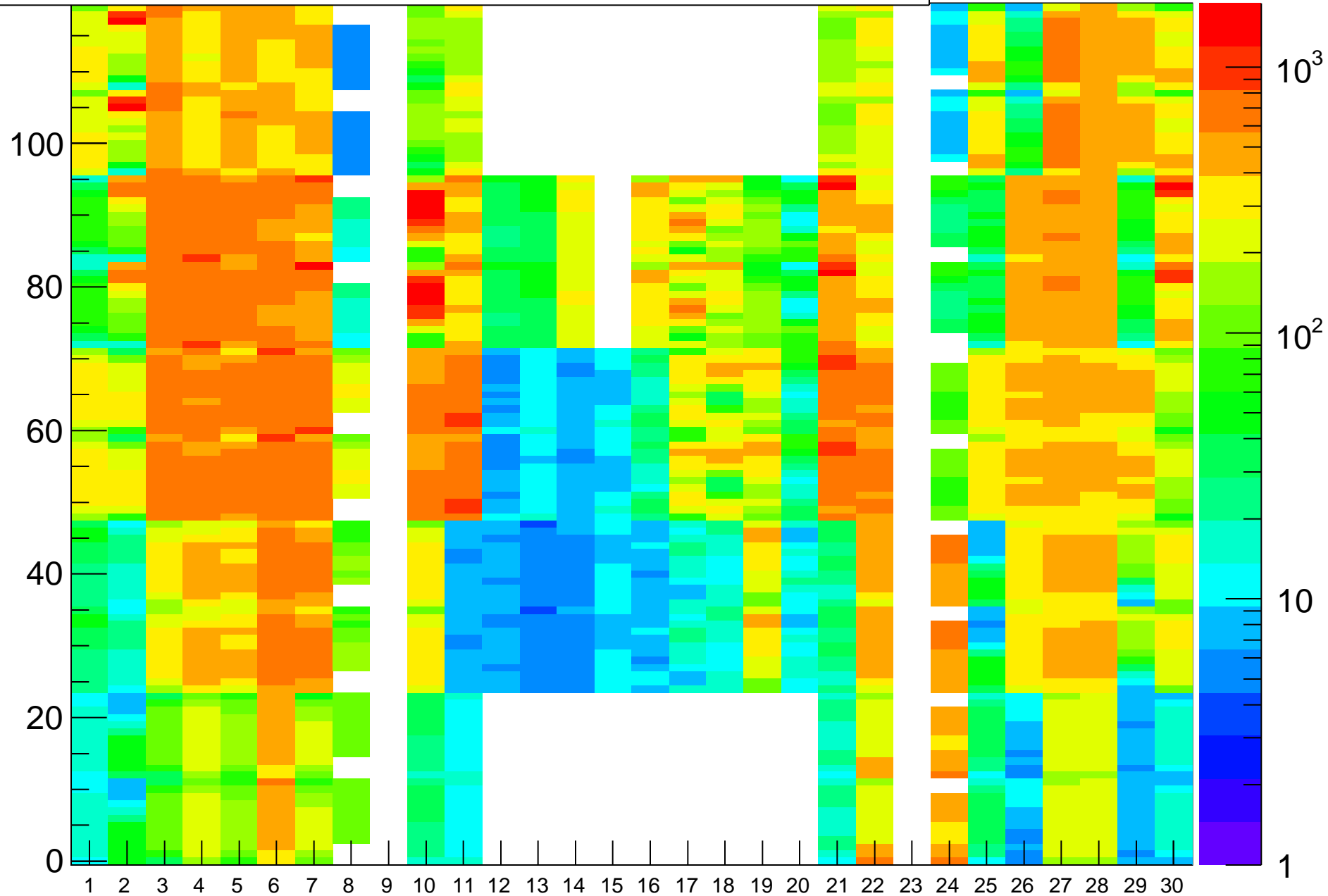
Rate (Hz) vs (BL,strip-posn), Run=15154
