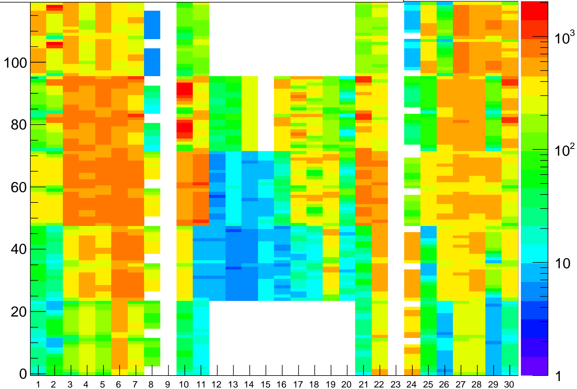
Rate (Hz) vs (BL,strip-posn), Run=15164
