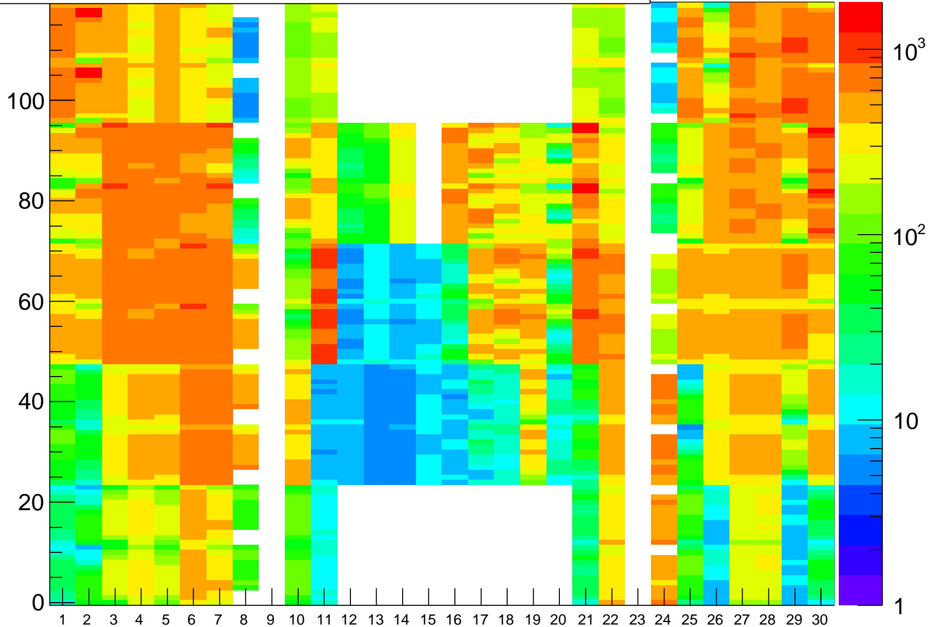
Rate (Hz) vs (BL,strip-posn), Run=15186
