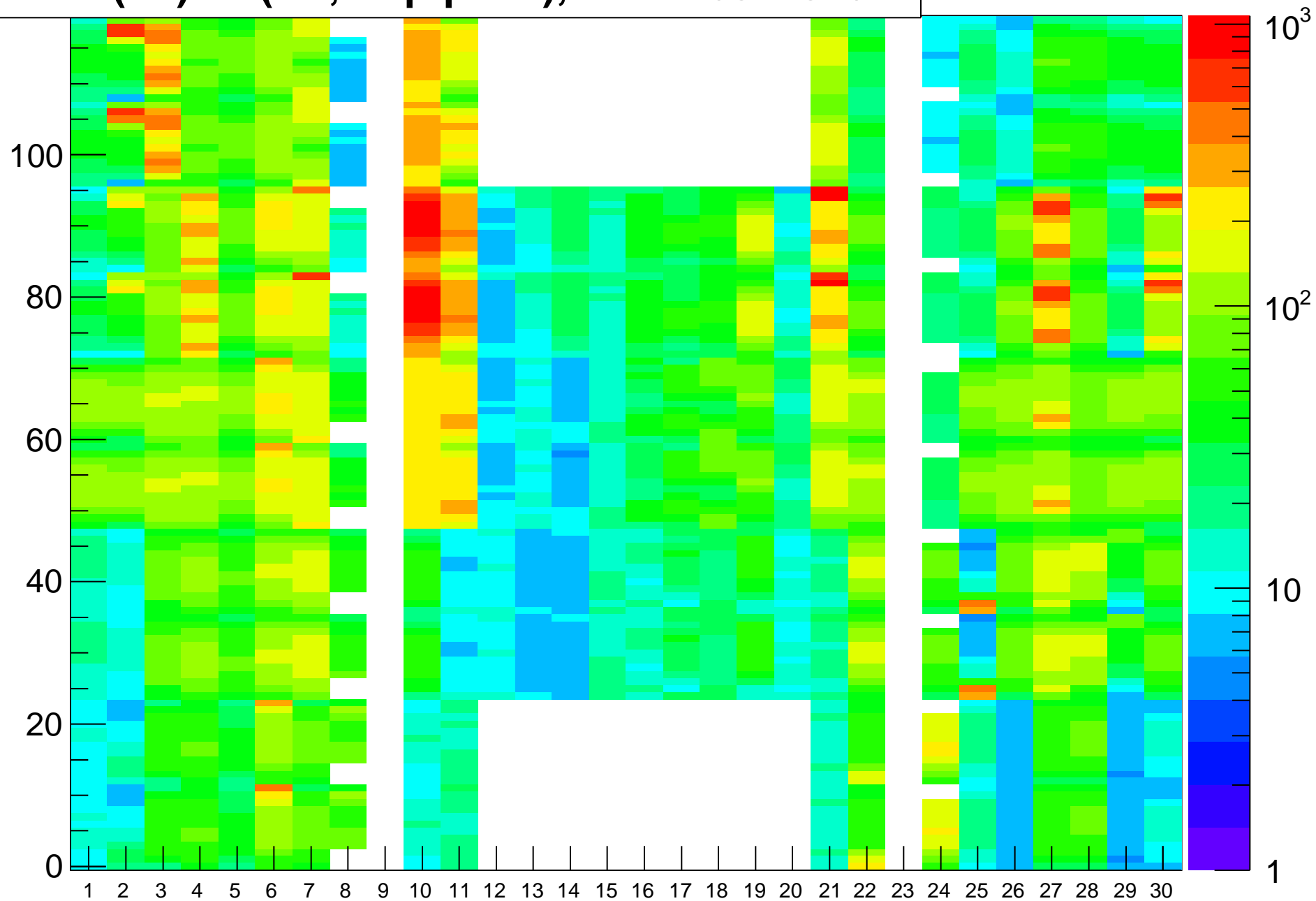
Rate (Hz) vs (BL,strip-posn), Run=16024078
