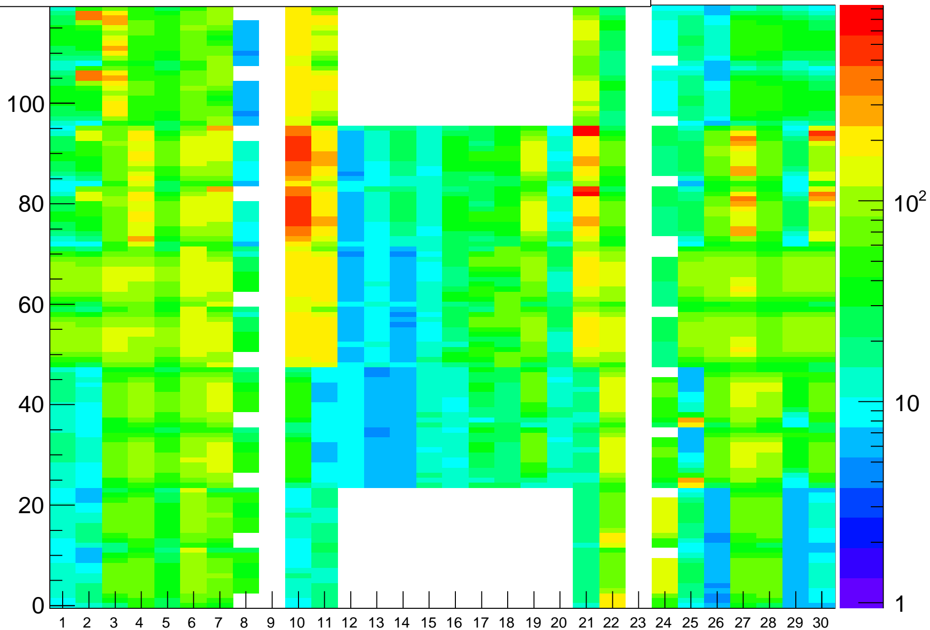
Rate (Hz) vs (BL,strip-posn), Run=16027011
