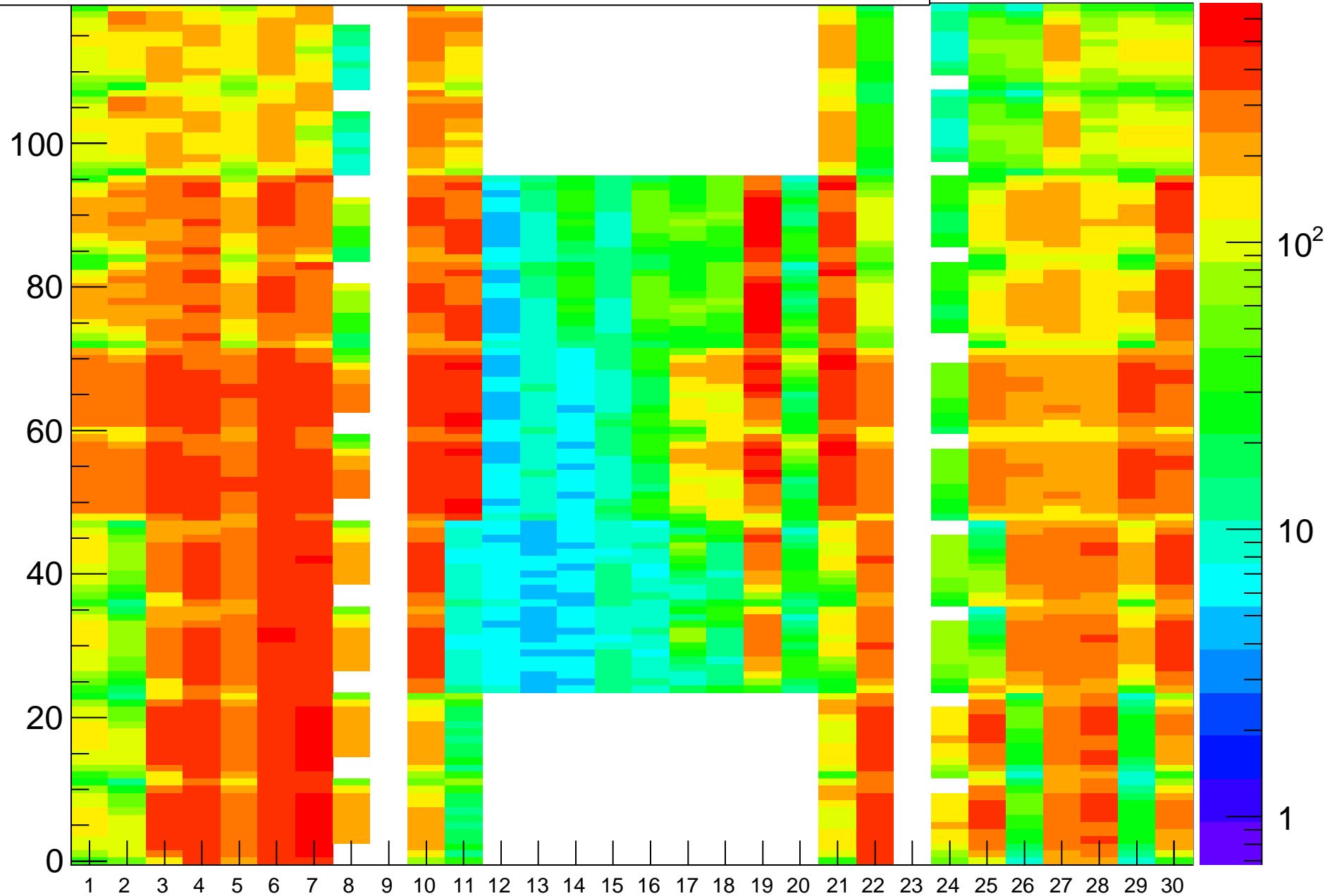
Rate (Hz) vs (BL,strip-posn), Run=16096
