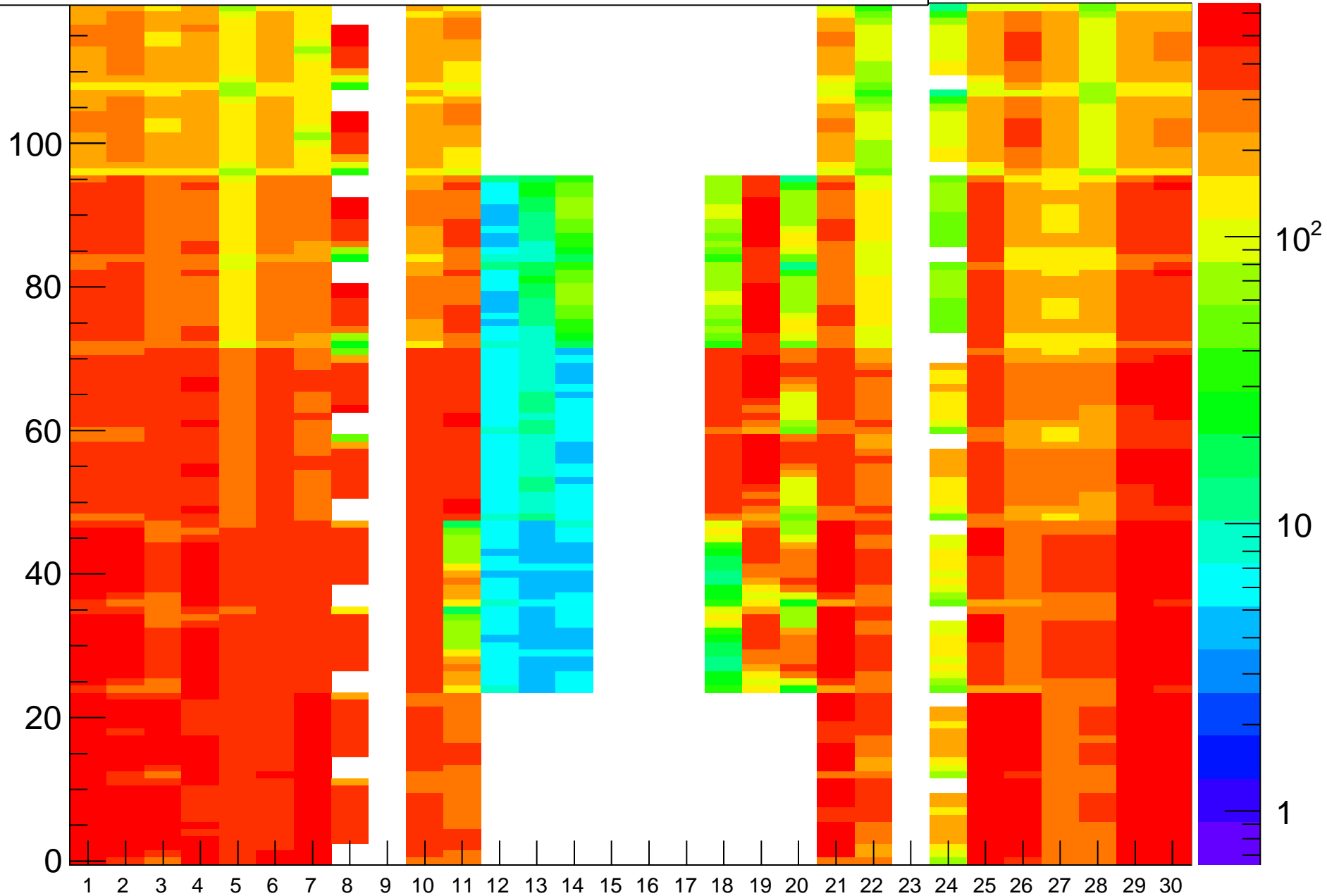
Rate (Hz) vs (BL,strip-posn), Run=16175
