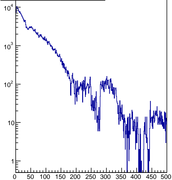
t-t_{\text{ear}}, n\text{Hits}/\text{tray}/\text{ev}>25
