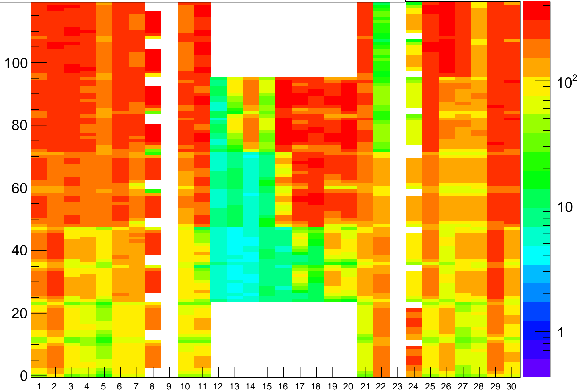
Rate (Hz) vs (BL,strip-posn), Run=17131
