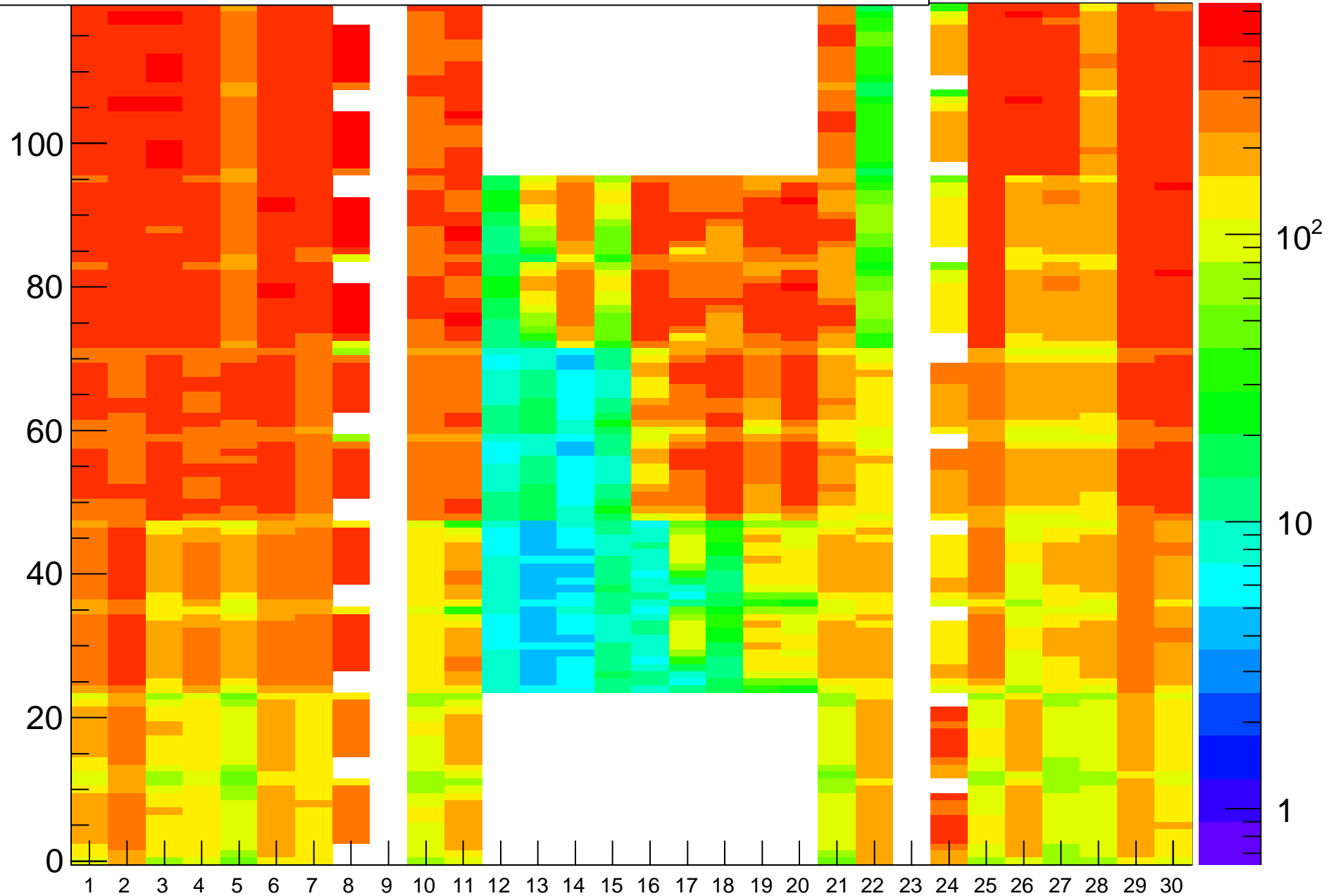
Rate (Hz) vs (BL,strip-posn), Run=17173
