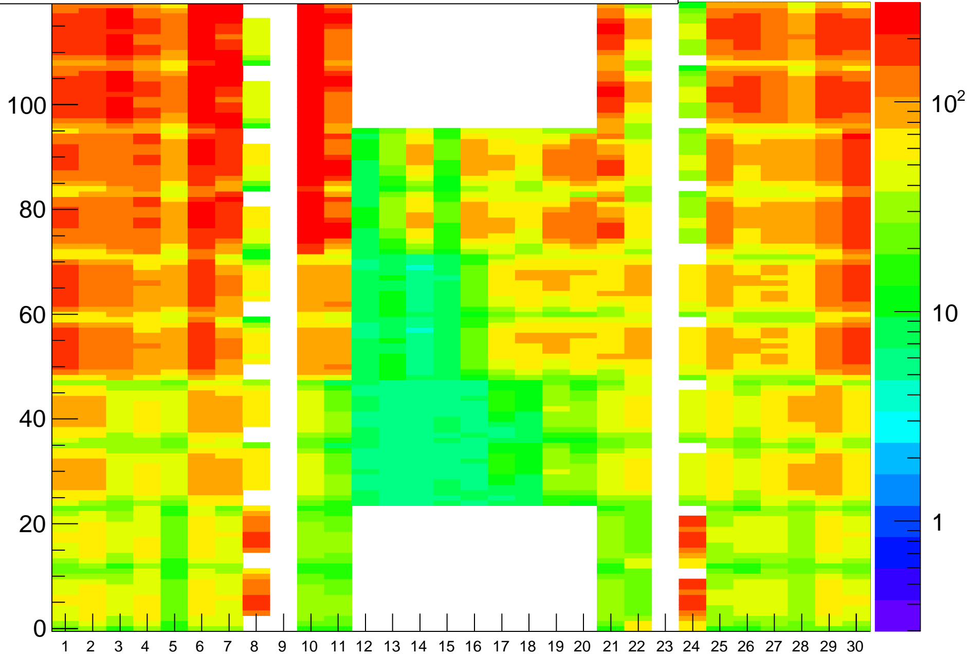
Rate (Hz) vs (BL,strip-posn), Run=18089
