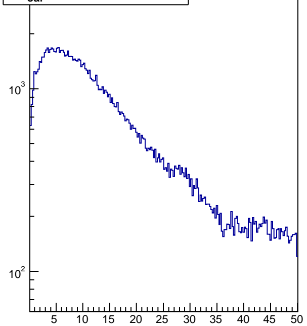
t-t_{\text{ear}}, n\text{Hits}/\text{tray}/\text{ev}>25
