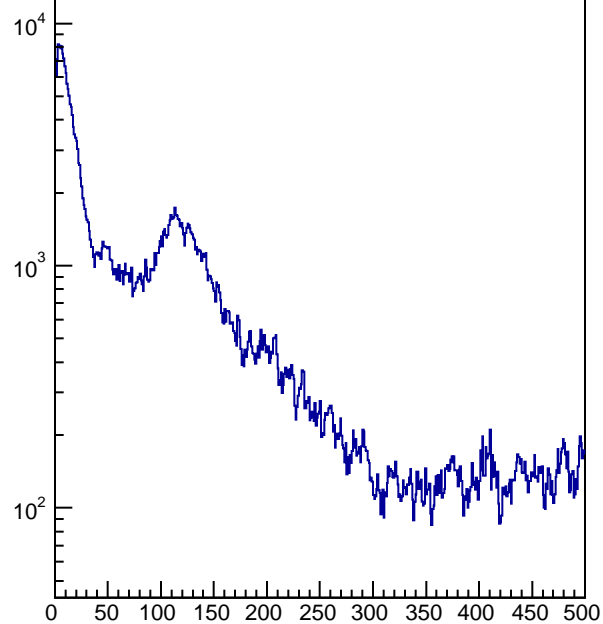
t-t_{\text{ear}}, n\text{Hits}/\text{tray}/\text{ev}>25
