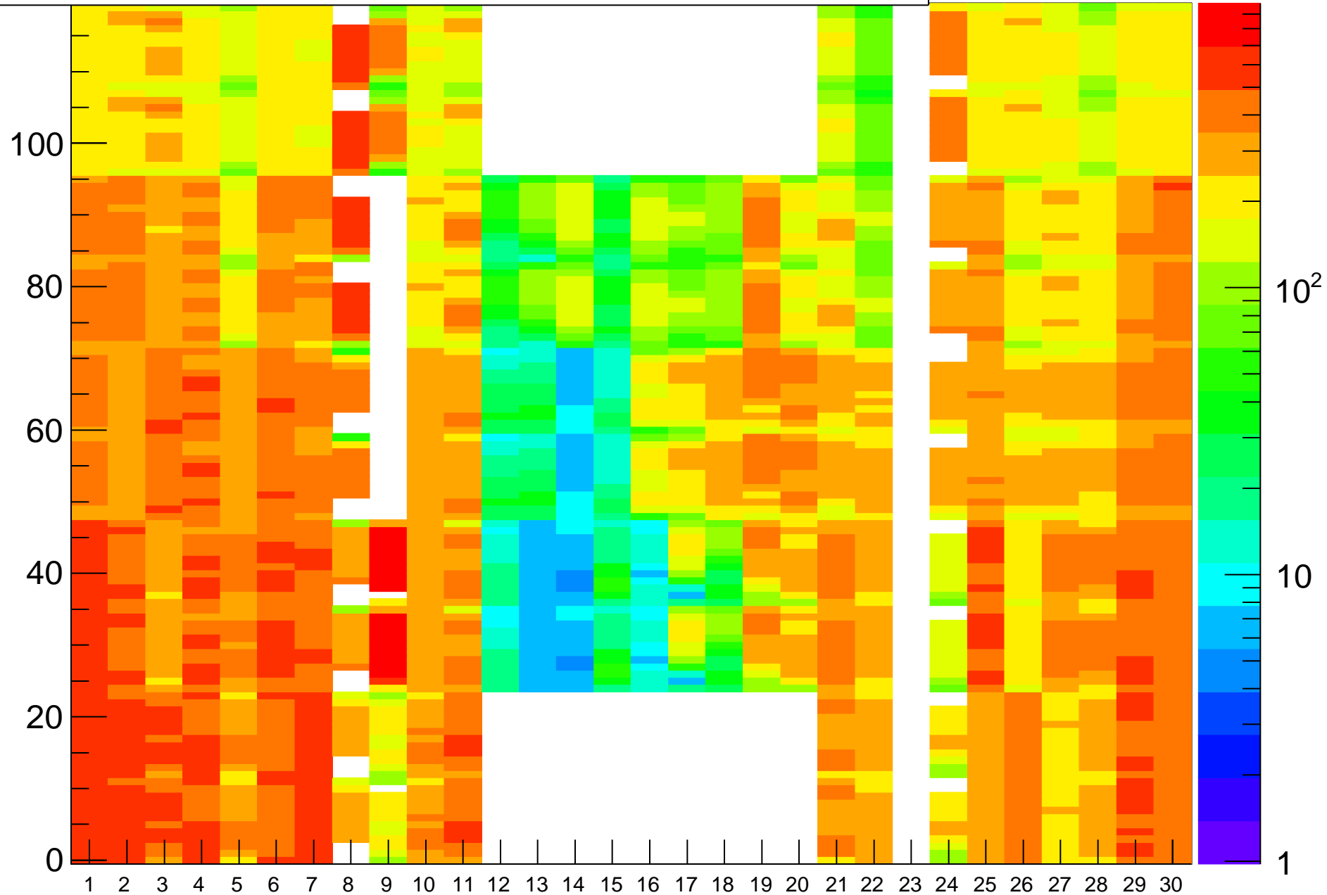
Rate (Hz) vs (BL,strip-posn), Run=18142
