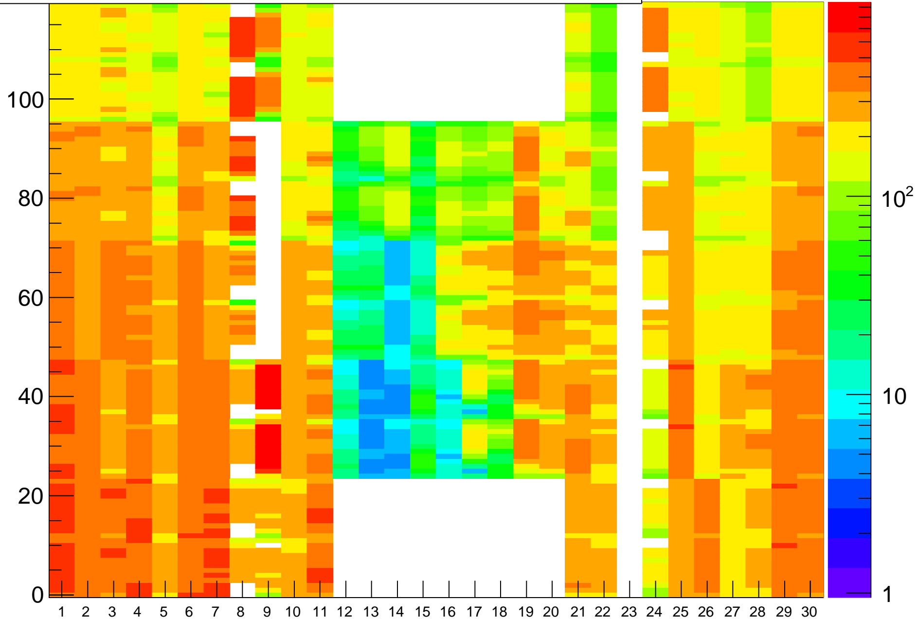
Rate (Hz) vs (BL,strip-posn), Run=18145
