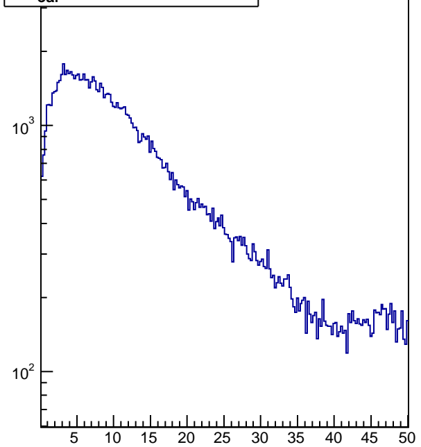
t-t_{\text{ear}} , nHits/tray/ev>25
