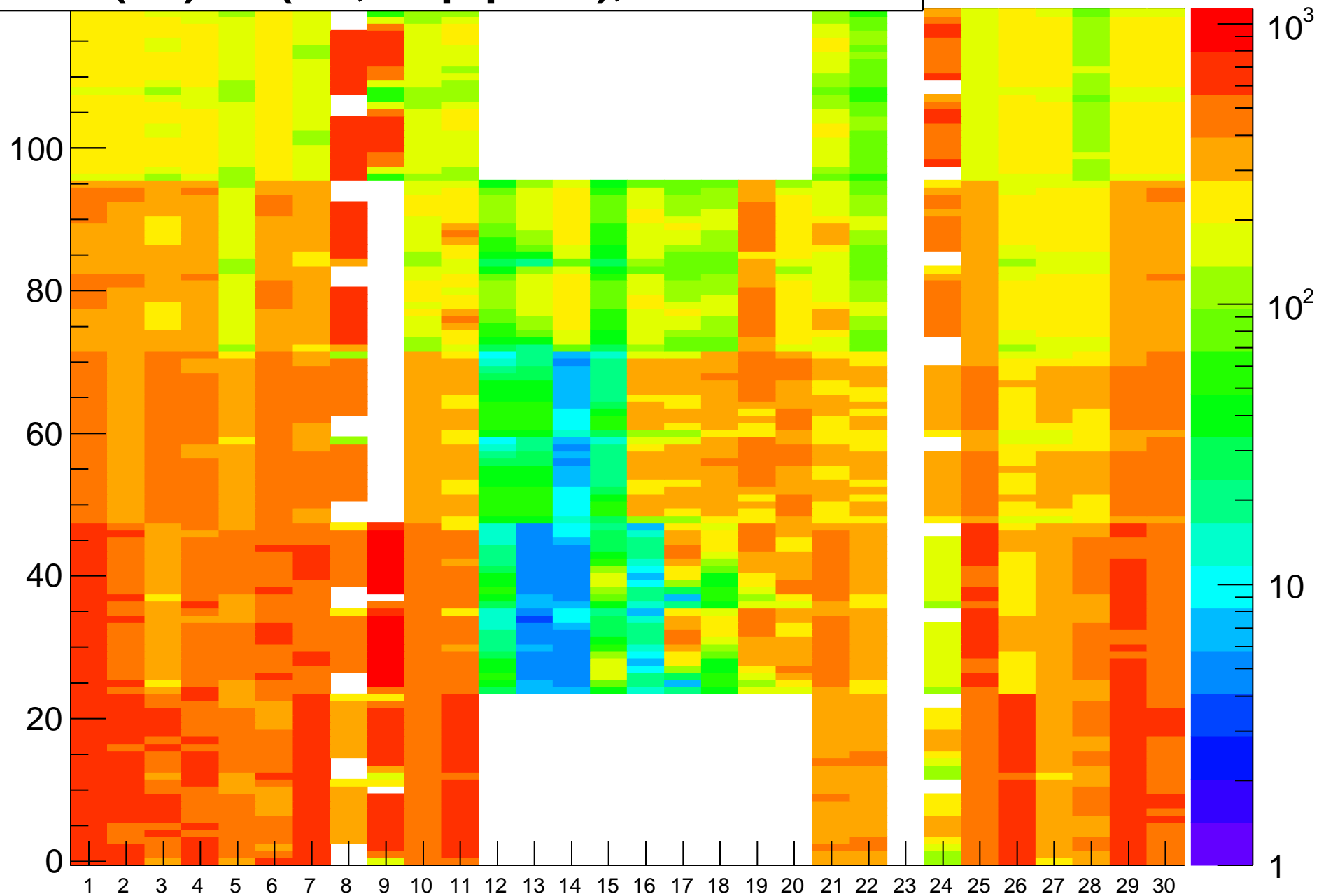
Rate (Hz) vs (BL,strip-posn), Run=18169
