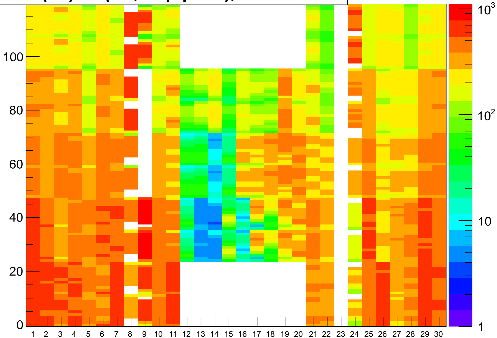
Rate (Hz) vs (BL,strip-posn), Run=18170
